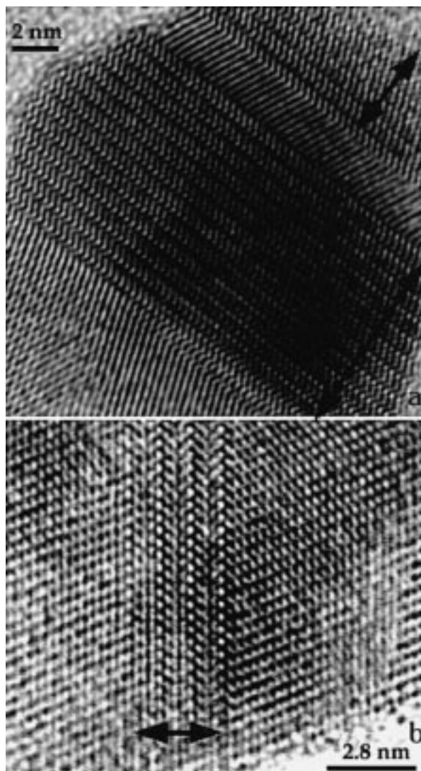
FIGURE 3. HRTEM images of anatase viewed down [131] and brookite down [011] . The boundary is anatase and (100) brookite. (a) domains of brookite (indicated by arrows) separated by anatase in twinned orientation; (b) three unit cell-wide strip of brookite in anatase.
