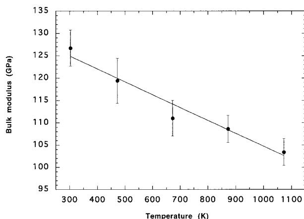
FIGURE 6. Bulk modulus of zoisite as a function of temperature. Bulk moduli are obtained from the Murnaghan fits in Figure 5. The best-fit straight line has the equation K_T = 125(3) - 0.029(6) (T - 298) GPa.
