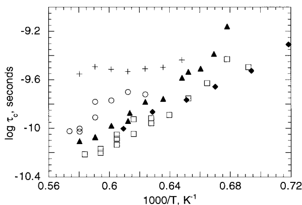
FIGURE 5. \log_{10} of correlation times calculated from NMR T_1 data plotted against the inverse of absolute temperature. Circles = CMAS2; triangles = Di; diamonds = NaMg2; squares = CMAS1; and crosses = KNM.
