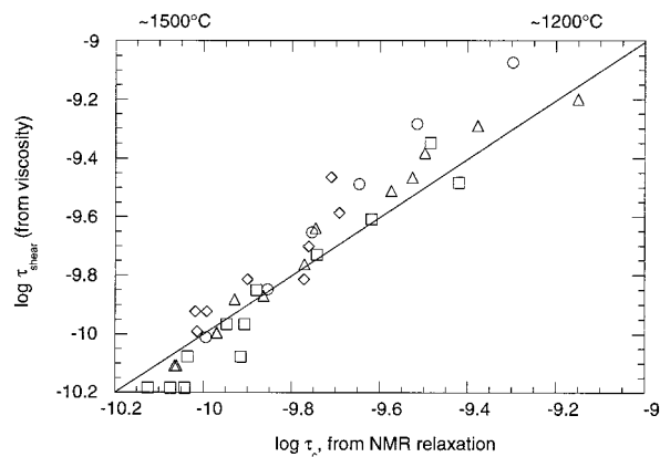
FIGURE 6. Comparison of \log_{10} \tau_{\text{shear}} calculated from viscosity data to \tau_c derived from ^{25}\text{Mg} NMR relaxation times in silicate melts. Circles = NaMg2; squares = CMAS1; triangles = Di; and diamonds = CMAS2. The line indicates where \tau_{\text{shear}} = \tau_c . Viscosity data from Bansal and Doremus (1986) and Ryan and Blevins (1987). Temperature labels indicate approximate ranges of these compositions for the correlation times shown.
