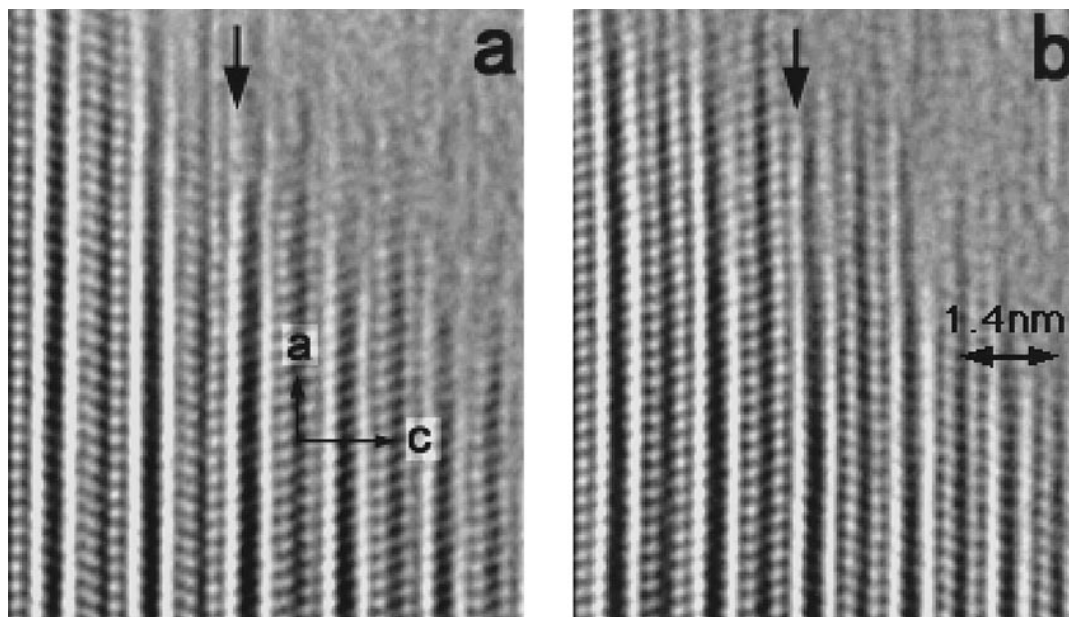
FIGURE 6. Filtered images of twinned Ibb chlorite from Tazawa mine showing two adjacent twin boundaries (a) in the left and (b) in the right. The arrows indicate the twin plane where I Ib stacking sequence forms.
