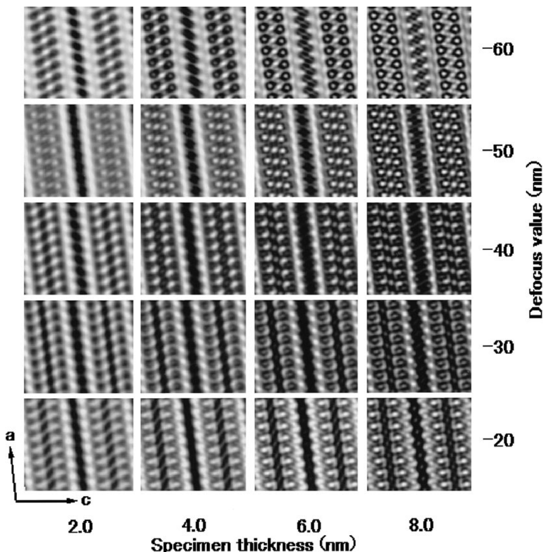
FIGURE 3. Simulated images for Ibb chlorite down [010] as functions of defocus and specimen thickness. The assumed composition at all octahedral sites is \text{Mg}_{0.5}\text{Fe}_{0.5} .
