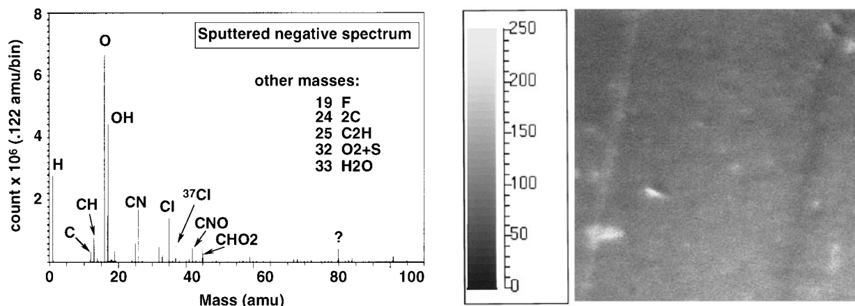
FIGURE 2. Negative mass spectrum corresponding to the positive spectra of Figure 1. Note that this is from the sputtered surface. The spectrum was collected for 30 min. Mass peaks are listed in Table. 1
