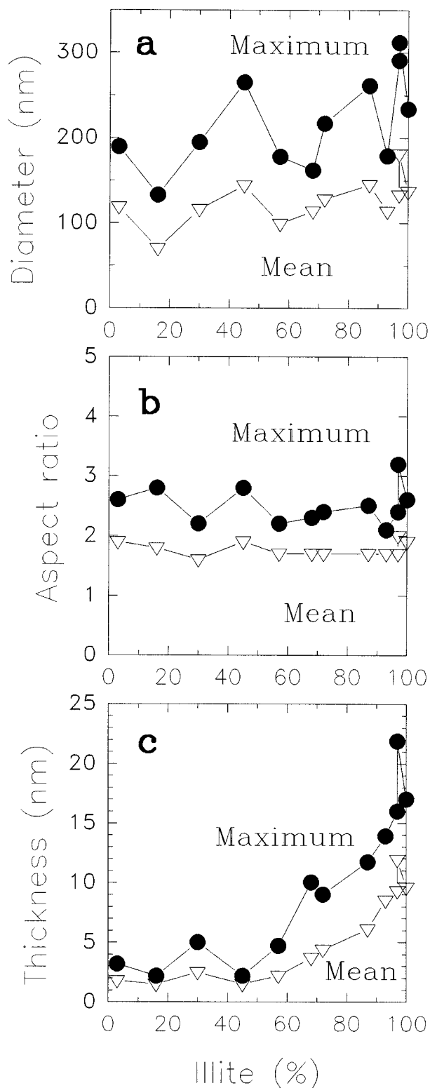
FIGURE 9. (a) Calculated diameter of particles ( \sqrt{1-w} ) vs. percent illite in I/S; (b) particle aspect ratio ( l/w ) vs. percent illite; (c) particle thickness vs. percent illite. Mean refers to average of all values. Maximum refers to the highest value, excluding the upper 10%. Only thickness shows a significant change with illitization.
