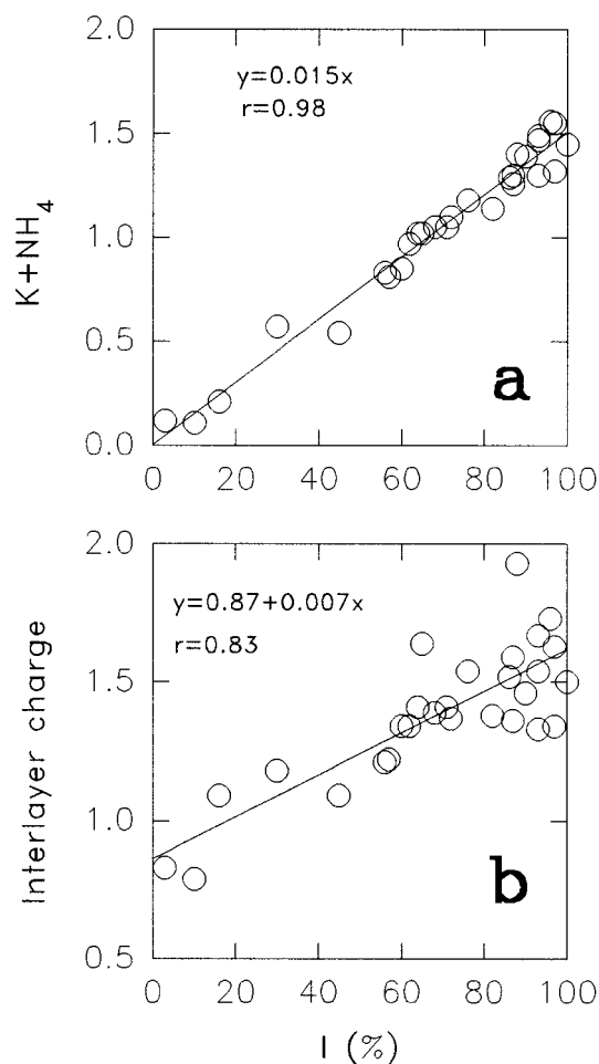
FIGURE 5. K + NH_4 content vs. percent illite in I/S (a) and interlayer charge vs. percent illite in I/S (b).
