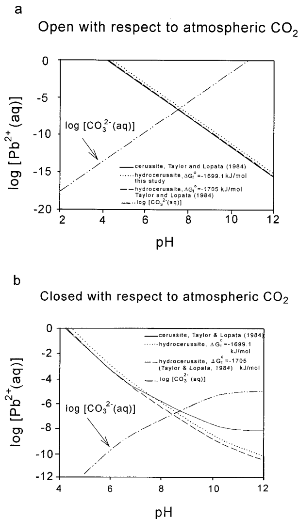
FIGURE 4. (a) The variation in the activity of \text{Pb}^{2+}(\text{aq}) as a function of \text{pH} at P_{\text{CO}_2} = 10^{-3.5} \text{ atm} for a solution that is open to exchange of \text{CO}_2 with the atmosphere. The lines correspond to \text{Pb}^{2+}(\text{aq}) activities in equilibrium with cerussite and hydrocerussite with two \Delta G_f^\circ [\text{Pb}(\text{OH})_2 \cdot (\text{PbCO}_3)_2(\text{s})] values were used to illustrate the sensitivity of the result to the choice of thermodynamic data for hydrocerussite. The variation in the activity of \text{CO}_3^{2-}(\text{aq}) is also shown. As one can see, hydrocerussite is always more soluble than cerussite, which is thermodynamically more stable. (b) The variation in the activity of \text{Pb}^{2+}(\text{aq}) as a function of \text{pH} with a total dissolved carbonate concentration of 10^{-5} \text{ m} for a solution that is closed to exchange of \text{CO}_2 with the atmosphere. The lines correspond to \text{Pb}^{2+}(\text{aq}) activities in equilibrium with cerussite and hydrocerussite; the variation in the activity of \text{CO}_3^{2-}(\text{aq}) is also shown. Hydrocerussite becomes considerably less soluble than cerussite at \text{pH} > 7 where the P_{\text{CO}_2} values are greatly reduced from 10^{-3.5} \text{ atm} .
