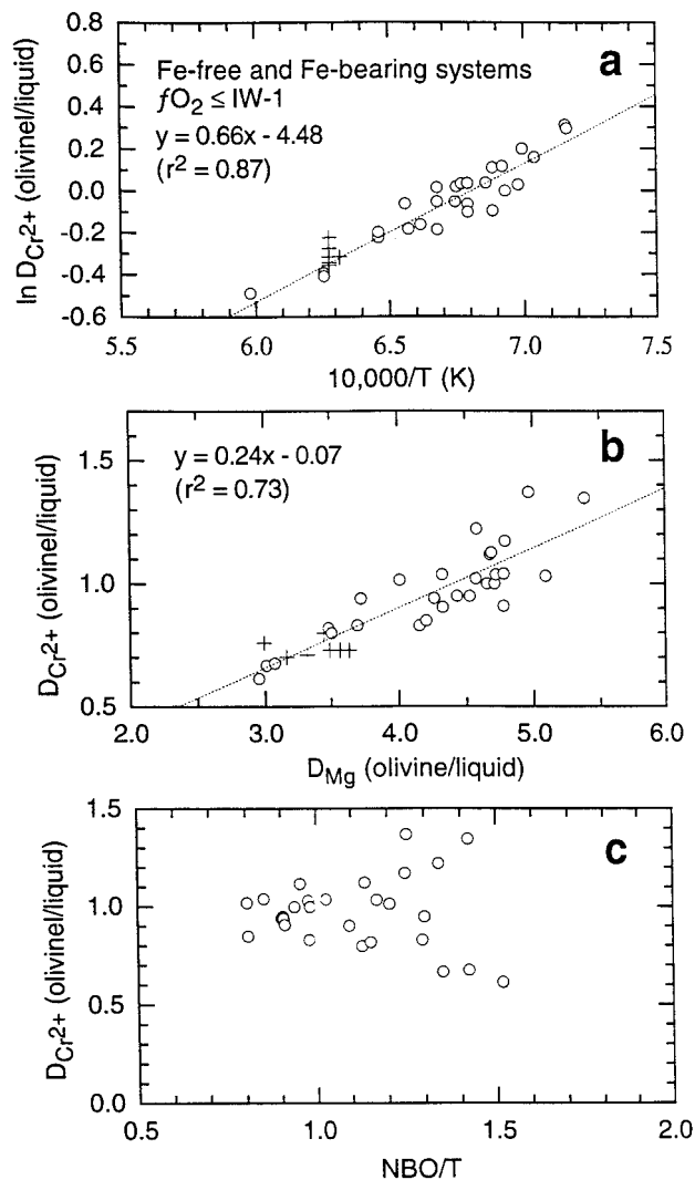
FIGURE 14. Plot of (a) \ln D_{Cr^{2+}} vs. 10,000/T(K) and (b) D_{Cr^{2+}} vs. D_{MgO} for Fe-bearing (circles) and Fe-free (crosses) experiments from this study and from the literature. We assume that, under these redox conditions, all of the Cr is divalent. The regression equations for these data are shown on the diagrams. Note the good covariation of D_{Cr^{2+}} with both of these parameters. (c) Plot of NBO/T vs. D_{Cr^{2+}} for the same Fe-bearing data sets shown in a and b. Note that, in contrast to D_{Cr^{3+}} , D_{Cr^{2+}} shows no systematic variation with NBO/T.
