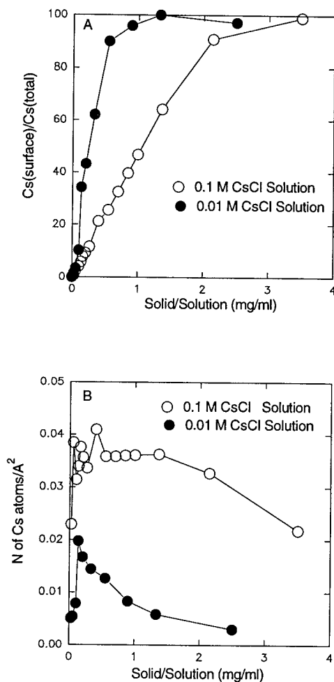
FIGURE 2. (A) Calculated surface Cs/total Cs ratio vs. solid/solution ratio for illite/CsCl solution mixtures. (B) Calculated Cs surface density on illite (atoms/ \text{\AA}^2 ) vs. solid/solution ratio for illite-CsCl solution mixtures. The first three data points in B and the first data point in A are for samples in which the solids settled to the bottom of the sample tube. For these samples the observed T_1 represents a larger but unknown solid/solution ratio.
