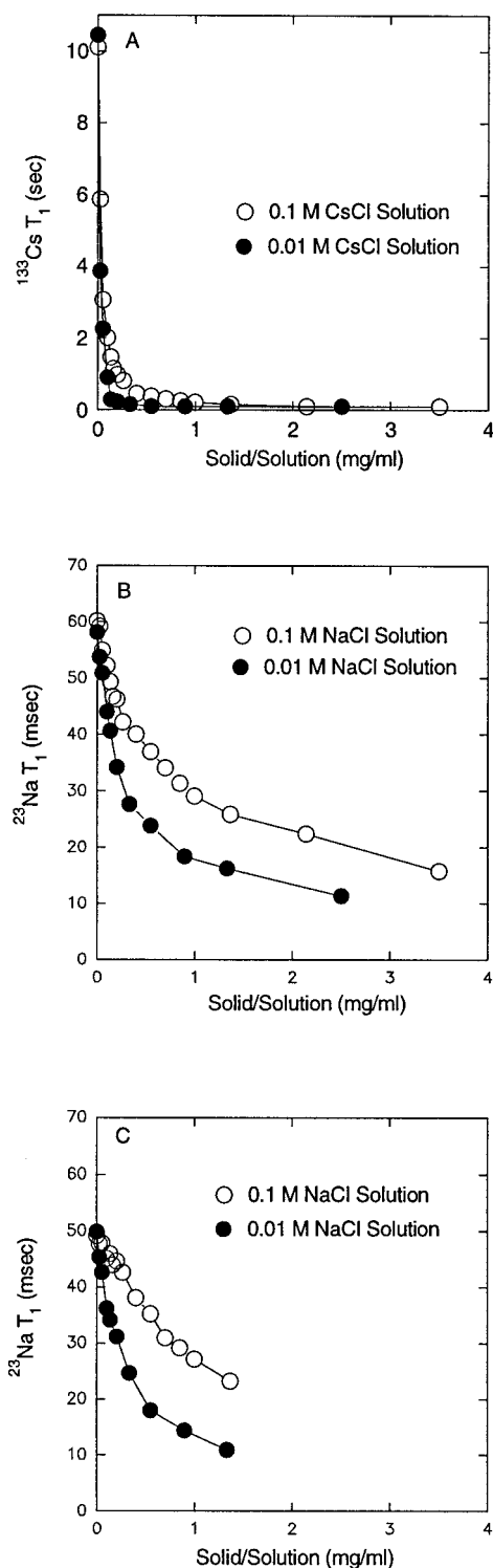
FIGURE 1. NMR T_1 relaxation times vs. solid/solution ratio for (A) ^{133}\text{Cs} in illite-CsCl solution mixtures, (B) ^{23}\text{Na} in illite-NaCl solution mixtures, and (C) ^{23}\text{Na} in silica gel-NaCl solution mixtures.
