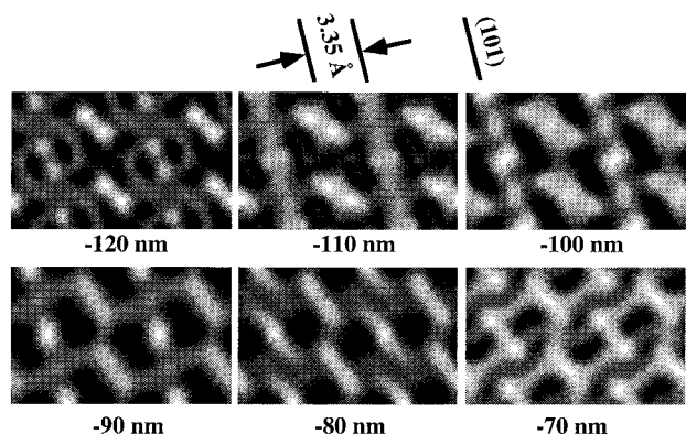
FIGURE 4. Calculated [111] zone axis HRTEM image of moganite (see text for detail).
