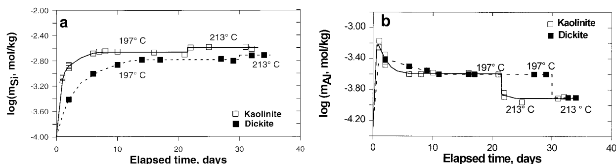
FIGURE 2. The evolution of solution compositions for kaolinite and dickite dissolution experiments at 197 and 213 °C: (a) aqueous Si concentration, (b) aqueous Al concentration.
