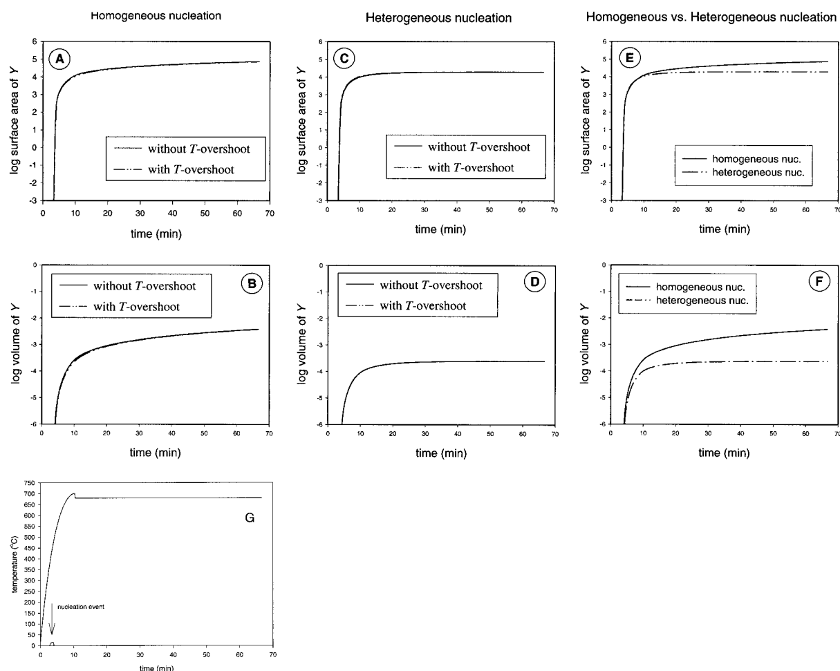
FIGURE 8. Results of the simulation, assuming that the product Y (quartz) is growing on the surface of the reactant X (silica gel), and assuming a heating procedure with a short temperature overshoot; (A and B) Development of the surface area and the volume of Y as f(t) for the fast heating procedure with T overshoot (— · — · —), and without T overshoot (—), assuming homogeneous nucleation. (C and D) The same as in A and B,
