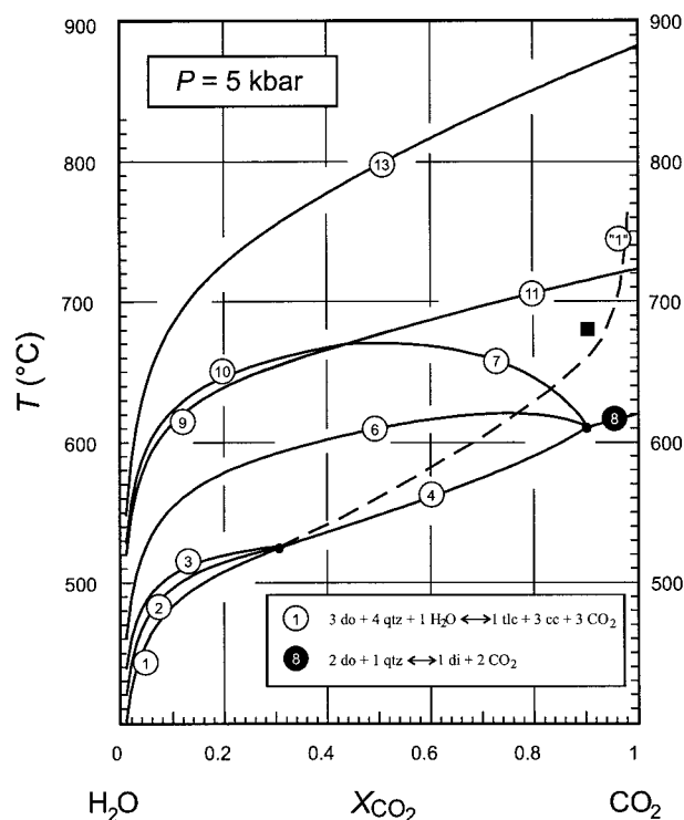
FIGURE 1. Isobaric- T - X_{\text{CO}_2} diagram showing reactions occurring in the system \text{CaO-MgO-SiO}_2\text{-CO}_2\text{-H}_2\text{O} (Fig. 8.14 in Gottschalk 1990). Curve 1 represents the equilibrium conditions of the reaction: 3 \text{ do} + 4 \text{ qtz} + 1 \text{ H}_2\text{O} = 1 \text{ tl} + 3 \text{ cc} + 3 \text{ CO}_2 , and the dashed line labeled 1 corresponds to its metastable extension. Curve 8 represents the reaction: 1 \text{ do} + 2 \text{ qtz} \leftrightarrow 1 \text{ di} + 2 \text{ CO}_2 . The black square indicates experimental T - X_{\text{CO}_2} conditions. Curve 13 represents the reaction: \text{cc} + \text{qtz} = \text{wo} + \text{CO}_2 studied by Tanner et al. (1985); for a complete list of reactions see Figure 4 in Gottschalk (1997). Abbreviations: cc = calcite, di = diopside, do = dolomite, qtz = quartz, tl = talc, wo = wollastonite.
