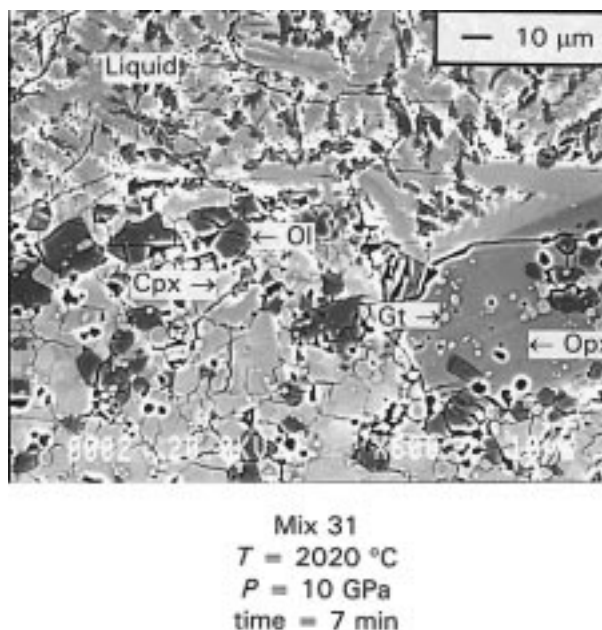
FIGURE 2. Backscatter scanning electron microscope image of an experiment on mix 31. Liquid quenches to form olivine, orthopyroxene, clinopyroxene, and garnet. Olivine, orthopyroxene, clinopyroxene, and garnet are all in contact with liquid.
