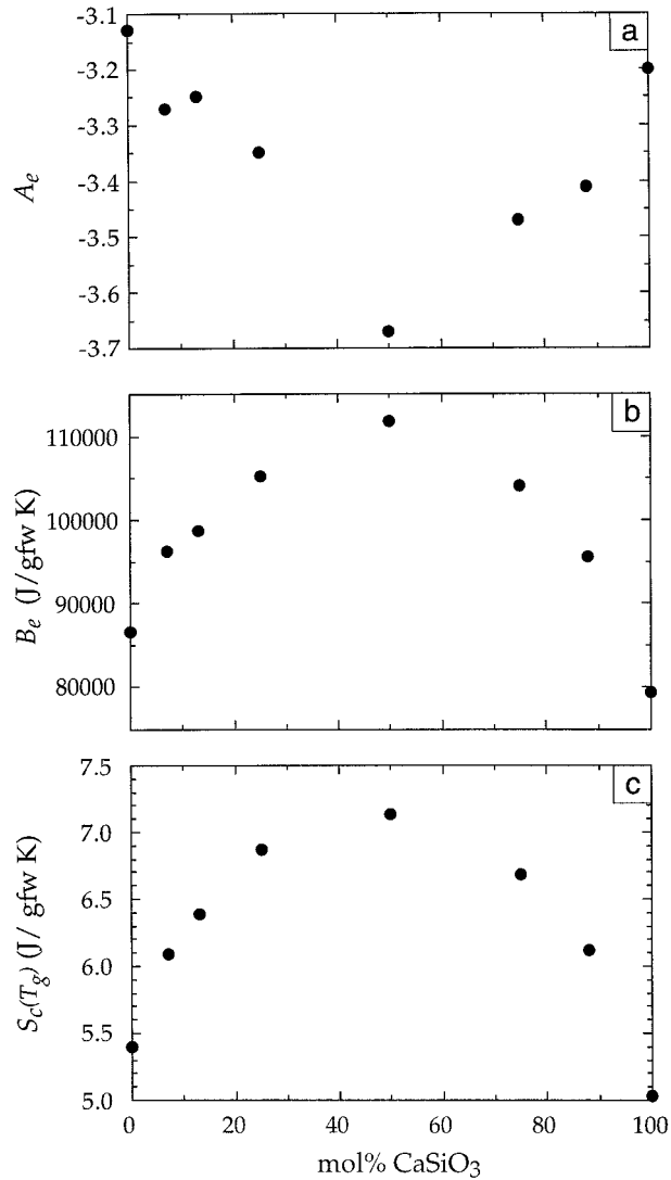
FIGURE 1. Variation of (a) A_e , (b) B_e , and (c) S_c(T_g) for the system \text{CaSiO}_3\text{-MgSiO}_3 (Neuville and Richet 1991; values per gram formula weight) showing the highly non-linear variation of these parameters, even in compositionally simple joins of constant polymerization.
