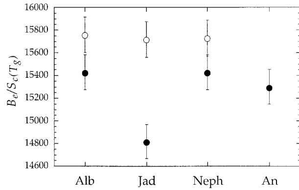
FIGURE 2. Variation of B_e/S_c(T_g) for “fully polymerized” aluminosilicates. Alb = NaAlSi 3 O 8 ; Jad = NaAlSi 2 O 6 ; Neph = NaAlSiO 4 ; An = CaAl 2 Si 2 O 8 . Filled symbols calculated using viscosity data for compositions exactly along the join SiO 2 -NaAlSiO 4 . Open symbols calculated using viscosity data for compositions inferred to contain no non-bridging O atoms (see text for details). Error bar represents \pm 1\% .
