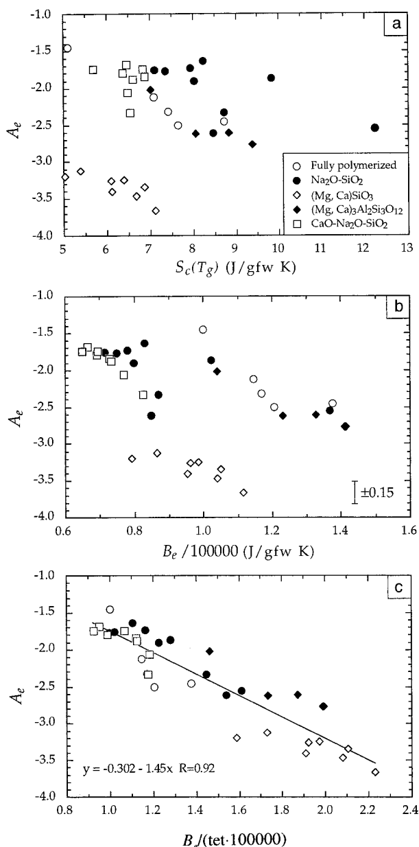
FIGURE 7. Variation of A_e for different compositions as a function of (a) S_c(T_g) ; (b) B_e ; and (c) B_e/\text{tetrahedron (Si + Al)} . Values are in gram formula weight. The error in individual values of A_e is approximately \pm 0.15 . The equation shown in (c) recovers values to within \pm 0.3 .
