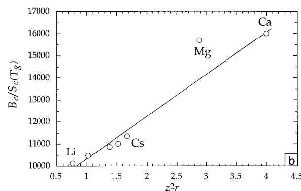
FIGURE 5. (a) Variation of B_e/S_c(T_g) along the joins \text{CaSiO}_3\text{-MgSiO}_3 (pyroxenes) and \text{Ca}_3\text{Al}_2\text{Si}_3\text{O}_{12}\text{-Mg}_3\text{Al}_2\text{Si}_3\text{O}_{12} (garnets). An error bar of \pm 1\% is shown. (b) Values of B_e/S_c(T_g) for Ca- and Mg-bearing compositions compared with alkali-bearing compositions as a function of z^2r ( z = ionic charge; r = ionic radius. See text for details).
