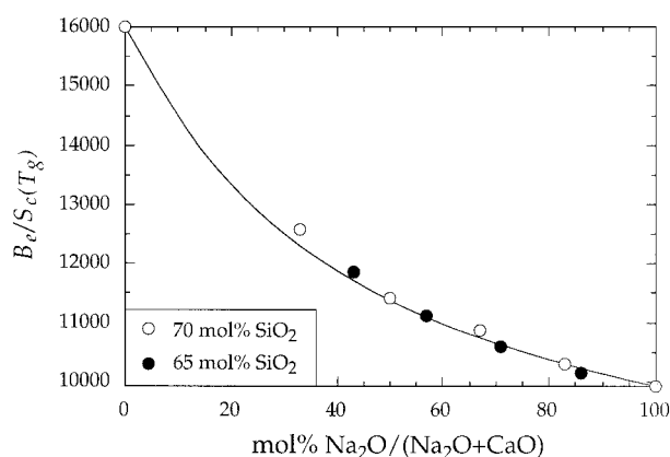
FIGURE 6. Variation of B_e/S_e(T_g) along the 65 and 70 mol% \text{SiO}_2 isopleths in the system \text{Na}_2\text{O}-\text{CaO}-\text{SiO}_2 . The solid line was calculated using Equations 13 and 16, and values of B_e/S_e(T_g)_{\text{NBO-Ca}} = 16\,000 ; B_e/S_e(T_g)_{\text{NBO-Na}} = 9950 ; and \{\phi_{\text{NBO-Na}}/\phi_{\text{NBO-Ca}}\} = 0.31 (see text for details).
