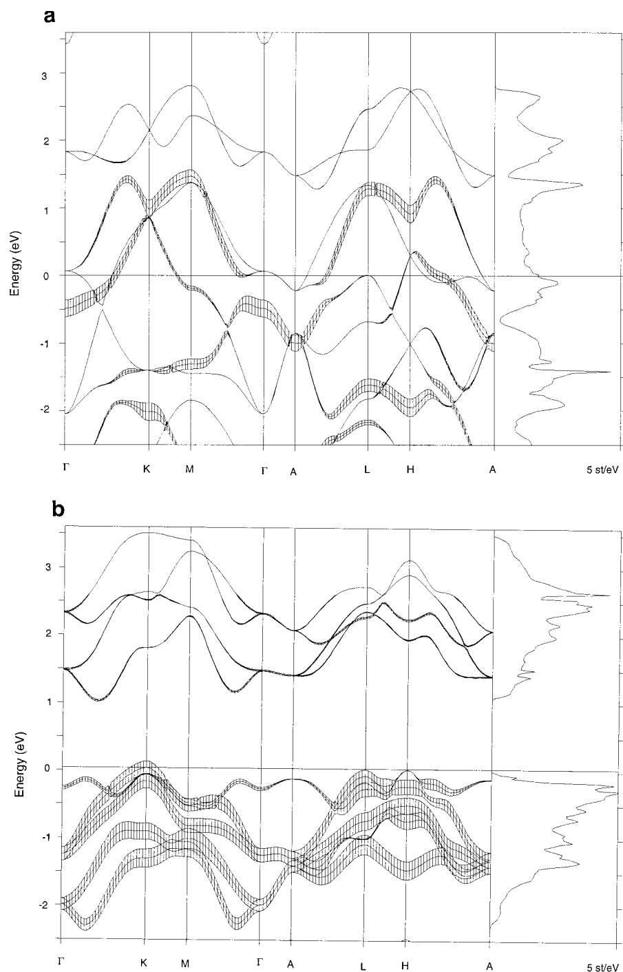
FIGURE 5. Band structures and densities of states at V = 14.8 \text{ \AA}^3 ( P \approx 96 \text{ GPa} ) computed using the LMTO-ASA method. The hatching width of the band represents the amount of spin-up character on one Fe. (a) B8 structure. This is a good metal due to the Fe-Fe interactions across the shared faces that leads to broad 3z^2-r^2 states, and broadening of the spin occupations. (b) Anti-B8 structure. This is a good insulator with a very wide gap. The spin-up states are much narrower and are almost fully occupied on one Fe atom per cell. The density of states is per spin.
