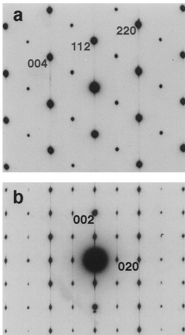
FIGURE 2. SAED patterns of (a) luzonite and (b) enargite obtained from [110]_{\text{luz}} and [100]_{\text{en}} . The diffuse streaks along [112]^*_{\text{luz}} and [001]^*_{\text{en}} indicate disorder in both structures. Streaks along 0kl with k = 3n are less pronounced than in other reciprocal lattice rows of enargite.
