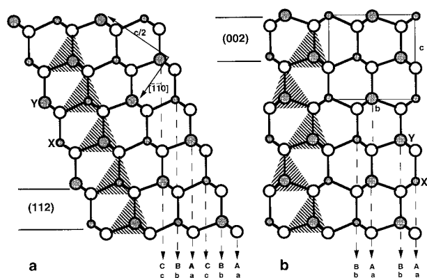
FIGURE 1. The structures of (a) luzonite and (b) enargite as projected along [110]_{\text{luz}} and [100]_{\text{en}} . Open circles = S atoms; filled circles = metal atoms. X and Y mark two types of metal-atom columns along the direction of projection; in X columns (small circles) there are only Cu atoms, whereas in Y columns (big circles) Cu and As atoms alternate.
