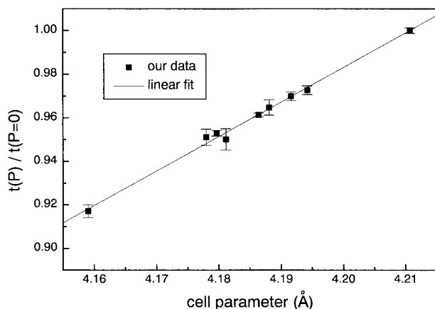
FIGURE 6. Normalized travel time t(P)/t(P = 0) vs. cell parameter. t(P) is the travel time at high pressure, t(P = 0) travel time at zero pressure. The straight line is a linear fit through the points. No ruby pressure measurement is involved in this plot. The uncertainties of the cell parameters are smaller than the symbols.
