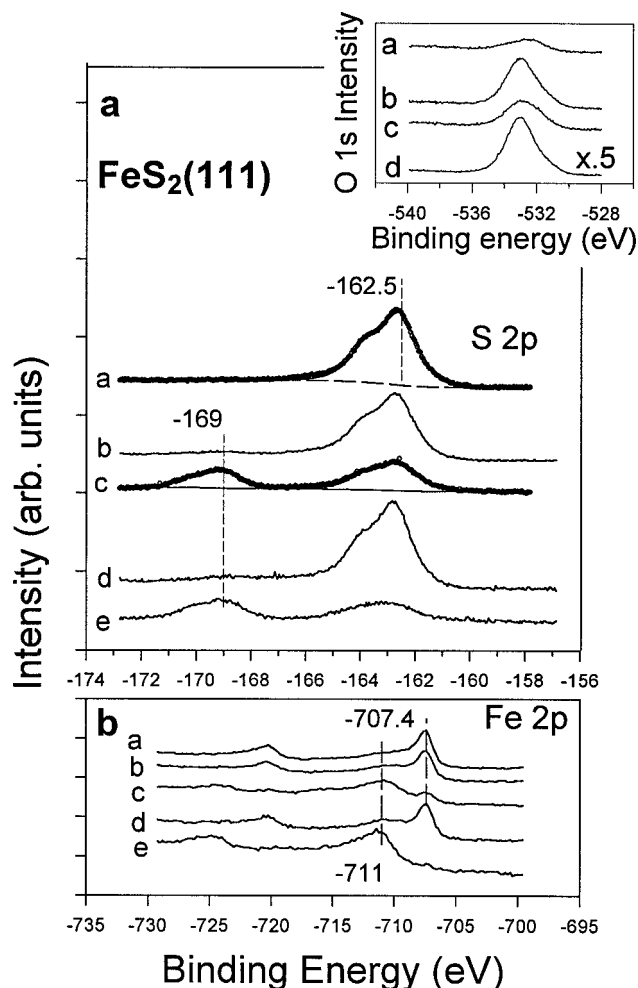
FIGURE 3. S 2p ( top ) and Fe 2p ( bottom ) data of FeS 2 (111) after (a) acid-washing, (b) exposure to 20 h of H 2 O vapor, (c) 200 h of H 2 O vapor, (d) 20 h of O 2 , and (e) 20 h of a H 2 O vapor/O 2 mixture. The inset exhibits O 1s data for FeS 2 (111) after (a) acid-washing, (b) 20 h of H 2 O vapor, (c) 20 h of O 2 , and (d) 20 h of a H 2 O vapor/O 2 mixture.
