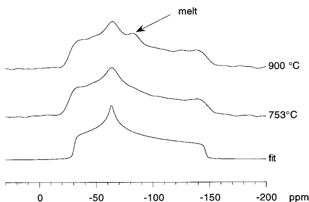
FIGURE 6. Static ^{29}\text{Si} spectrum of \text{Na}_2\text{SiO}_3 at 753 °C (bottom) and 900 °C (top) under \text{N}_2 -5% \text{H}_2 , showing the appearance of a narrow melt peak near -82 ppm.
