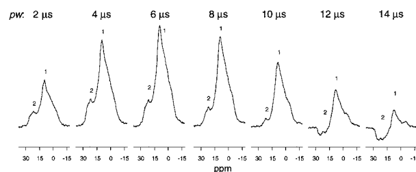
FIGURE 4. ^{23}\text{Na} spectra of \text{Na}_2\text{SiO}_3 at 783° C obtained using different pulse rf widths p_w . Seven spectra are shown, with scales in ppm. Two sites with different 180° (inversion) times can be seen, as also shown in Figure 3; peak 2 is nulled and inverted at slightly shorter pulse lengths than peak 1.
