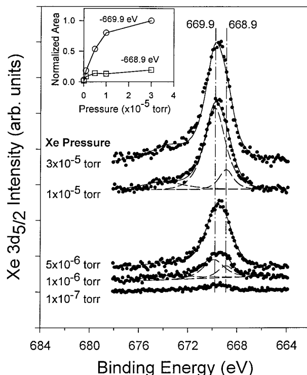
FIGURE 1. PAX data for atomically clean \text{FeS}_2(100) as a function of the Xe background pressure. These data were obtained at a sample temperature of 79 \text{ K} . The 669.9 and 668.9 \text{ eV} features are thought to be associated with Xe adsorbed on stoichiometric and defect surface, respectively. The inset plots the area of these two PAX features as a function of Xe pressure.
