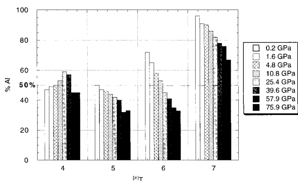
FIGURE 8. Aluminum fractionation of ^{[4]}\text{T} , ^{[5]}\text{T} , ^{[6]}\text{T} , and ^{[7]}\text{T} . Percentage of aluminum for a given ^{[n]}\text{T} is given as the percentage of all ^{[n]}\text{T} coordinated subunits that are aluminum for all time steps in a simulation experiment. For dominant ^{[n]}\text{T} , i.e., ^{[4]}\text{T} at low pressure and ^{[6]}\text{T} , ^{[7]}\text{T} at the higher pressures, the number of subunits found across the entire simulation is usually >15\,000 . For non-dominant ^{[n]}\text{T} , there is usually <3000 subunits for the entire simulation.
