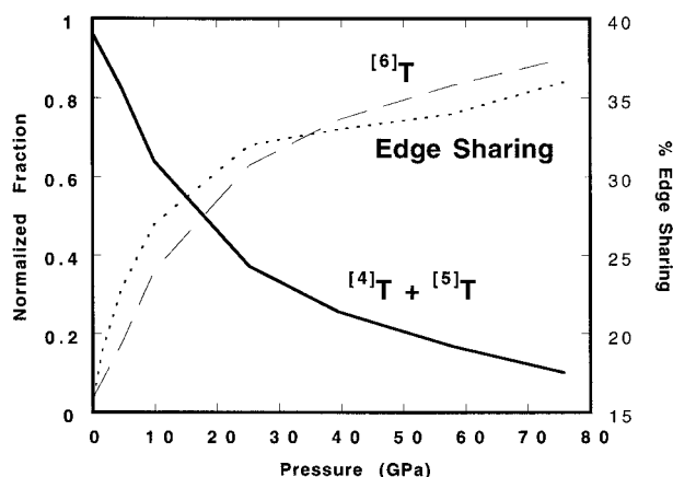
FIGURE 3. The calculated number fraction abundance of ^{[6]}T (dashed curve) and ^{[4]}T + ^{[5]}T (solid curve) normalized to unity and plotted against pressure at 4000 K for \text{CaAl}_2\text{Si}_2\text{O}_8 . Dotted curve, the number fraction of edge-sharing \text{TO}_n polyhedra. The correlation of the fraction of polyhedra that take part in edge sharing with abundance of ^{[6]}T is consistent with the distribution of T-O-T angles in Figure 2.
