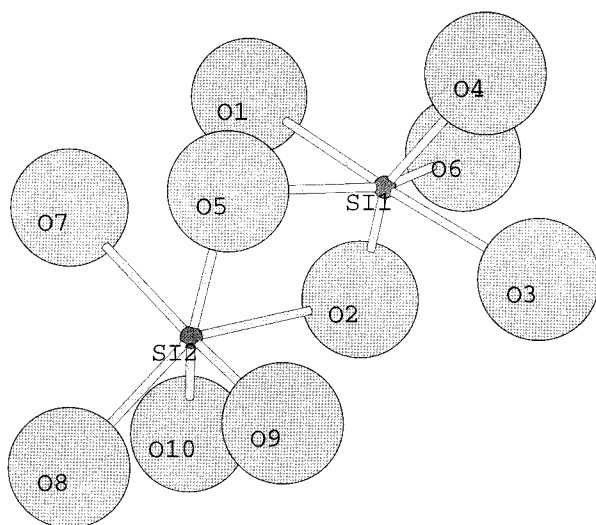
FIGURE 5. Oblique view of a pair of edge-sharing [6]T from an MD simulation at 25.3 GPa and 4000 K. The O-T-O angle O_5-Si_1-O_2 is 89.4^\circ and the O-T-O angle O_5-Si_2-O_2 is 73.7^\circ . The Si-O-Si angle is either 101^\circ ( Si_1-O_5-Si_2 ) or 92.2^\circ ( Si_1-O_2-Si_2 ). The ions O2, O4, O5, O6, O8, and O10 are approximately coplanar.
