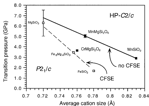
FIGURE 3. Transition pressures of the P_{21/c} to HP C2/c transformation in clinopyroxenes plotted as a function of average cation radius. Error bars (only given if larger than symbol size) represent observed hysteresis loops. Transition pressures for \text{MgSiO}_3 and \text{FeSiO}_3 are taken from Angel et al. (1992) and Hugh-Jones et al. (1994), respectively, those of intermediate members of the (\text{Fe,Mg})\text{SiO}_3 series are taken from Ross and Reynard (1998, unpublished data) and are represented by a dashed line. Note that the transition pressure of clinopyroxenes containing \text{Fe}^{2+} or \text{Cr}^{2+} (crystal field stabilized ions) appear to be shifted to lower pressures.
