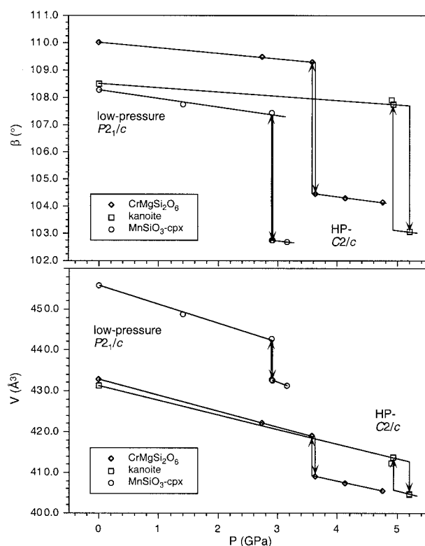
FIGURE 1. The variation of the unit-cell angle \beta and unit-cell volume with pressure in kanoite (squares), \text{MnSiO}_3 (circles), and \text{CrMgSi}_2\text{O}_6 (diamonds). The P_{21/c} to HP C2/c phase transition is indicated by a strong decrease of \beta and V at 5.06 \pm 0.14 GPa (kanoite), 2.905(5) ( \text{MnSiO}_3 ) and at 3.60 \pm 0.03 GPa ( \text{CrMgSi}_2\text{O}_6 ).
