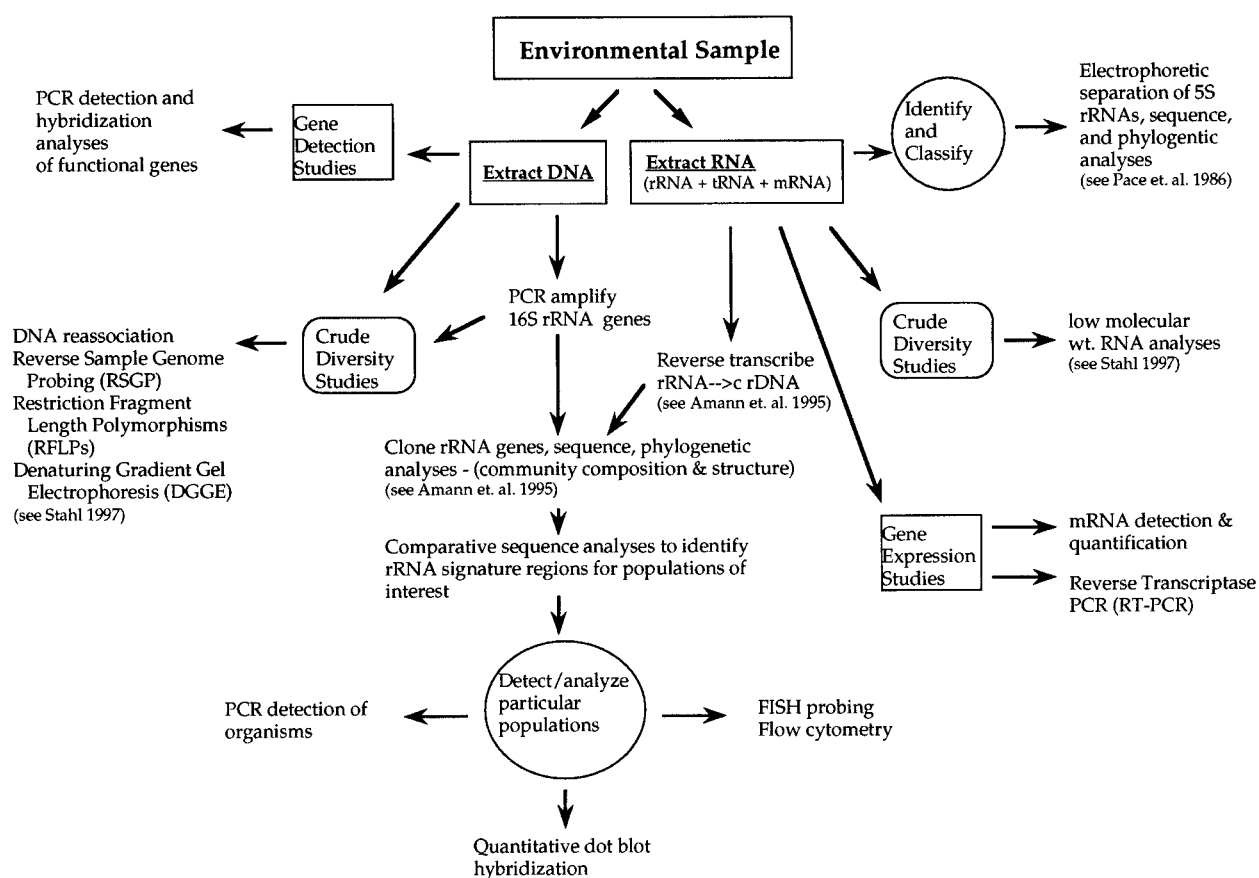
FIGURE 1. Flow chart of possible applications of nucleic-acid approaches to examine microorganisms in environmental samples. Once extracted from the environment, RNA and DNA can be used in investigations of microbial identity and taxonomic characterization, crude diversity studies, or an investigation of function by detection of functional genes (DNA), and/or the detection of gene expression (RNA). See the indicated references and text for details.
