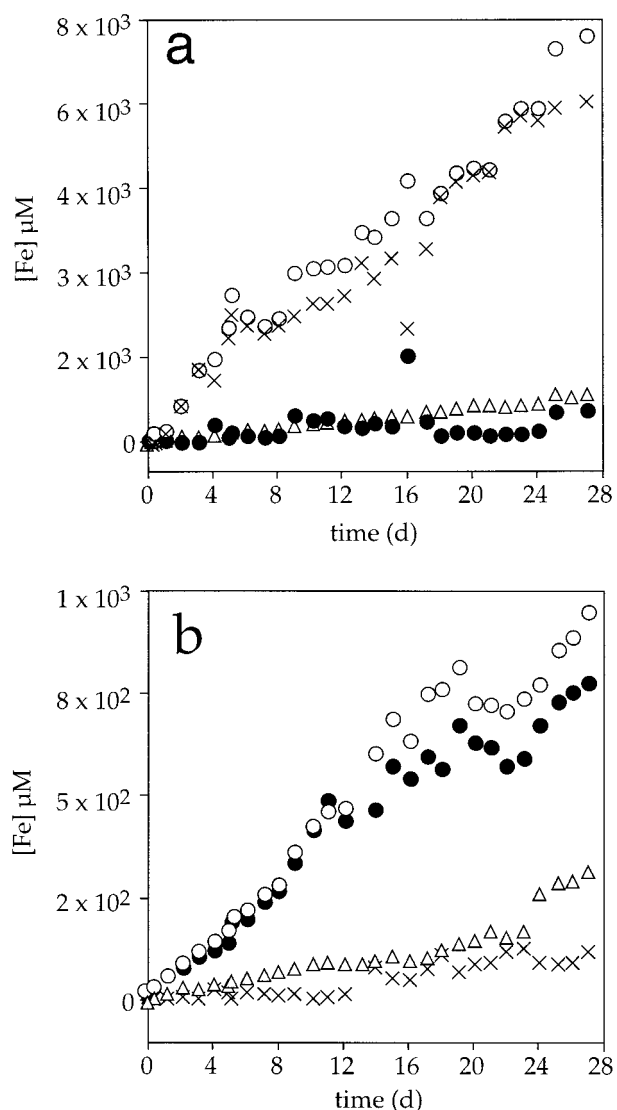
FIGURE 10. Iron speciation data for enrichment cultures containing organisms that attach to pyrite (a), and cultures that lack attaching phases (b). Symbols are as follows: open circles = total Fe released in enrichment cultures; triangles = total Fe released in corresponding control experiments; crosses and filled circles = Fe 3+ and Fe 2+ . Speciation is not shown for controls; in both cases, it was predominantly Fe 2+ .
