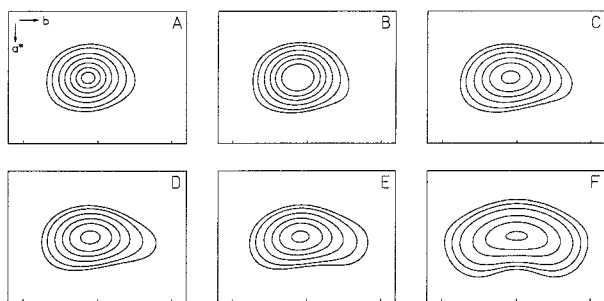
FIGURE 1. Electron-density maps for the Pb site viewed along the c axis; scale = 1 \text{ \AA} . (A) \text{PbF}_L (Benna et al. 1996). (B) \text{PbF}_L1h . (C) \text{PbF}_L16h . (D) \text{PbF}_L64h . (E) \text{PbF}_L136h . The contours drawn correspond to 20, 40, 80, 130, 180, and 240 \text{ e}^- \text{ \AA}^{-3} . (F) \text{PbF}_H (Benna et al. 1996). The coordinates of the center of the plots are: x = 0.27 , y = 0 , z = 0.07 for A, B, C, D, E, and z = 0.14 for F.
