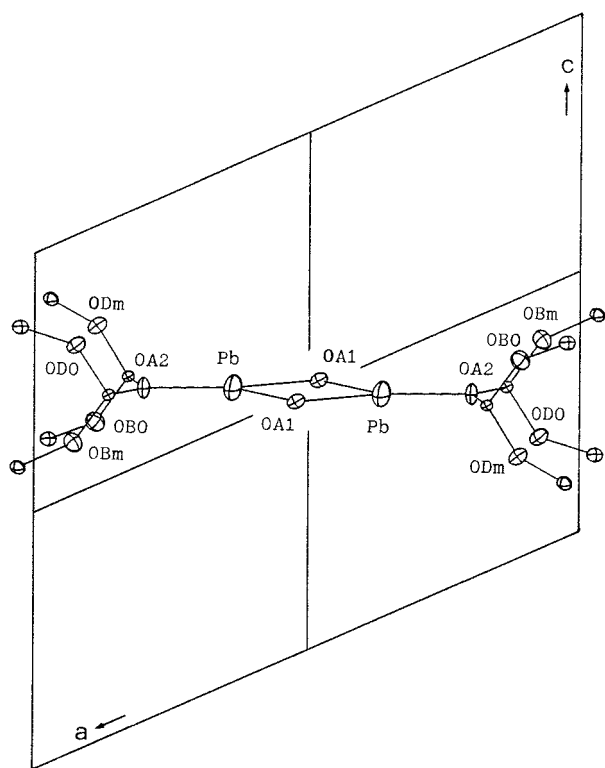
FIGURE 3. Partial projection on the (010) plane of \text{PbF}_H structure (e.g., C2/m , c = 7.174 \text{ \AA} ) (Benna et al. 1996). The projection was slightly rotated to avoid overlapping of atoms. T atoms are not labeled.
