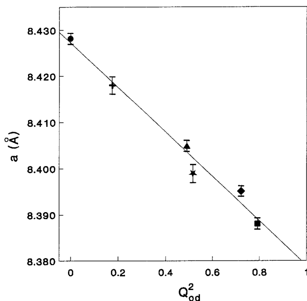
FIGURE 5. Value of the a unit-cell parameter vs. Q^2_{od} . Symbols as in Figure 2.
