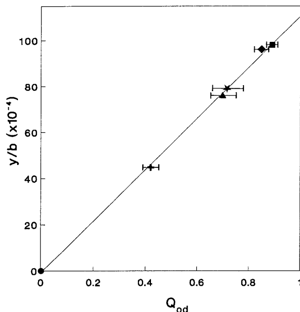
FIGURE 2. Absolute value of y/b fractional coordinate of the Pb site vs. Q_{\text{od}} . Circle and square = \text{PbF}_H and \text{PbF}_L , respectively (Benna et al. 1996); diamond = \text{PbF}_L1h ; star = \text{PbF}_L16h ; triangle = \text{PbF}_L64h ; cross = \text{PbF}_L136h .
