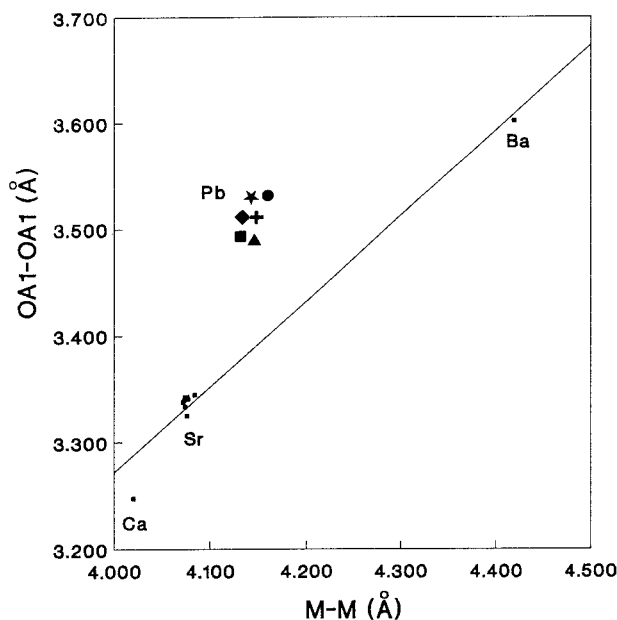
FIGURE 4. OA1-OA1 vs. M-M distances (see Fig. 3) in calcium feldspar (Wainwright and Starkey 1971), strontium feldspar (Chiari et al. 1975; Benna et al. 1995), lead feldspar (Benna et al. 1996; this work), and barium feldspar (Griffen and Ribbe 1976). Symbols as in Figure 2.
