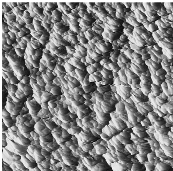
FIGURE 5. HAP reacted with 0 mg/L [Pb_{aq}] . TMAFM image of the reaction blank showed rounded features with the absence of crystallographically controlled dissolution features (scan area = 2.38 \mu\text{m} on a side). SEM and TEM of the same sample (results not shown) revealed that the HAP particle size decreased and its edges became rounded. XRD results were analogous to the reactant material (see Fig. 3b). EDS (results not shown) were similar to unreacted HAP, showing only Ca and P.
