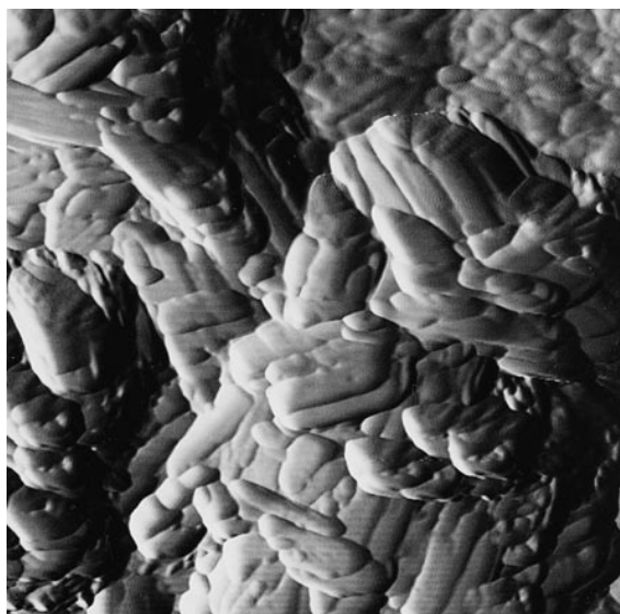
FIGURE 10. HAP reacted with 0.5 mg/L [Pb_{aq}]_i . TMAFM image showing a needle-like phase preferentially oriented on the surface of another phase (scan area = 1.60\ \mu\text{m} on a side). Coupled with other results, this is evidence of heterogeneous nucleation of a solid Pb phase on the surface of HAP. SEM, TEM, XRD, and EDS results (not shown) were similar to those of the reaction blank.
