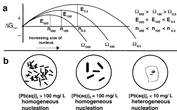
FIGURE 1. (a) Schematic illustration of the role of saturation on the competing processes of nucleation (increasing \Delta G_{\text{rxn}} ) and growth (decreasing \Delta G_{\text{rxn}} ) (modified after Berner 1981). As the degree of saturation is increased, there is a decrease in both the free energy barrier to nucleation and the size of the stable nucleus. (b) Predicted morphology of precipitates at various solution saturation states which, for HPY, are strongly dependent upon the initial aqueous Pb concentration ( [\text{Pb}_{\text{aq}}]_i ). ( \Delta G_{\text{rxn}} = Gibbs energy, \Omega = saturation state, E = activation energy, n = size of critical nucleus, subscripts refer to [\text{Pb}_{\text{aq}}]_i in mg/L).
