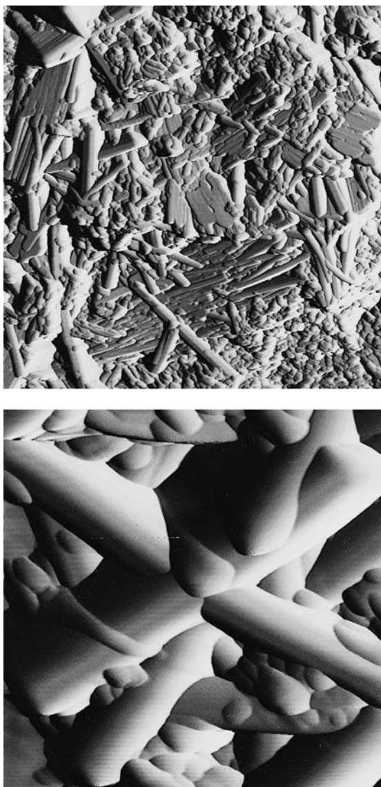
FIGURE 8. HAP reacted with 10 mg/L [Pb_{aq}]_i . (top) TMAFM image showing needles which appear to be preferentially oriented on another phase (scan area = 2.00 \mu\text{m} on a side). This is evidence in support of heterogeneous precipitation of HPY on the surface of HAP. (bottom) TMAFM image of an intergrowth with hexagonal symmetry (scan area = 700 nm on a side). SEM, TEM, EDS, and ED results (not shown) were similar to those at 100 mg/L [Pb_{aq}]_i . XRD pattern (see Fig. 3c) showed that the sample was dominated by HAP with lesser amounts of HPY.
