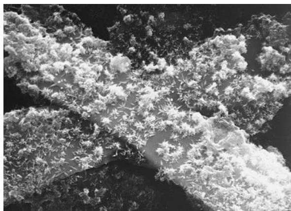
FIGURE 11. HAP reacted with 100 mg/L [Pb_{aq}]_i and allowed to age for several days. SEM image of needles of HPY (image size = 23 \times 16\ \mu\text{m} ). The needles of HPY grew significantly larger because of Ostwald ripening (compare with Fig. 8b); yet, some small needles remained as rosettes on the surface of these larger needles.
