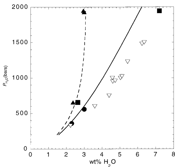
FIGURE 1. Comparison of Moore et al. (1995b) data for phonolite (solid triangles) with the data of Carroll and Blank (1997) (IR = upside-down open triangles; manometry = solid squares = 900 °C). The dashed line is the predicted H 2 O solubility from Moore et al. (1995b), and the solid line is from this study calculated for 900 °C. Note the severe underestimation of the Moore et al. (1995b) data and its subsequent effect on their model curve.
