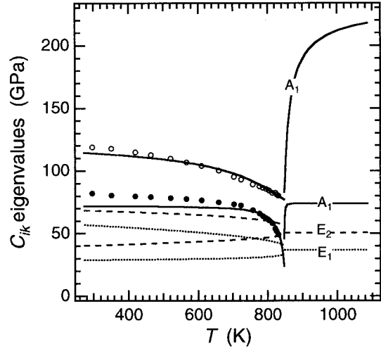
FIGURE 17. Variations of the eigenvalues of the elastic constant matrix for crystals with point group 622 ( T > T_{tr} ) and point group 32 ( T < T_{tr} ). Expressions for the eigenvalues of 622 crystals are given in Table 4. ( E_1 is plotted as C_{44} ; E_2 is plotted as C_{66} ). A_1 eigenvalues of crystals with 32 symmetry have the same form as those of crystals with 622 symmetry. The smooth curves were determined from the calculated variations shown in Figure 9 (data from solutions derived from assuming \Delta C_{11} = \Delta C_{12} and (\Delta C_{13})^2 = \Delta C_{11}\Delta C_{33} in \beta quartz). Solid lines represent the A_1 eigenvalues; broken and dotted lines represent the other eigenvalues. Each of the E_1 and E_2 eigenvalues of \beta quartz splits into two in \alpha quartz. Experimental data points for A_1 eigenvalues are shown below T_{tr} (data from Ohno 1995). There is reasonable agreement between calculated and experimental data over the complete temperature range for one of the A_1 eigenvalues and close agreement over the range T_{tr} to \sim 750 K for the other. Neither of the A_1 eigenvalues reaches zero at the transition point.
