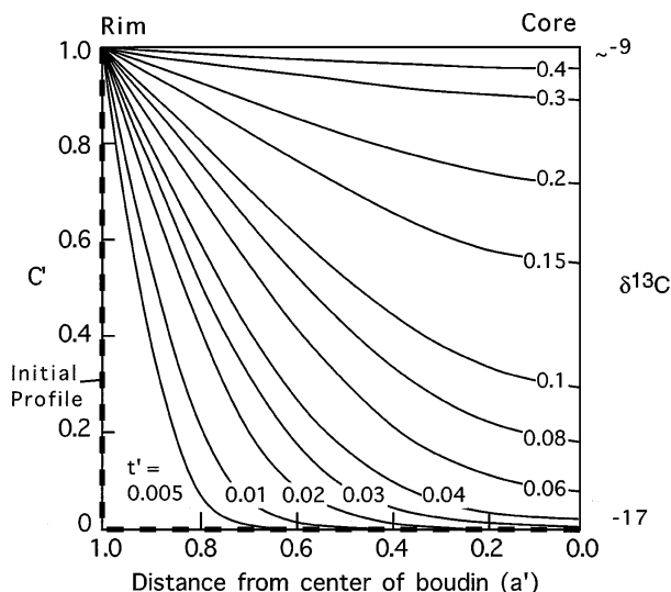
FIGURE 6. Geochemical profiles resulting from spherical diffusion at different dimensionless times, t' = (D_e t K_e^{-1}) / a^2 , where D_e is the effective diffusion coefficient, t is time, K_e is the rock-fluid partition coefficient and a is boudin radius. The profiles in Figure 5 resemble those predicted for spherical diffusion.
