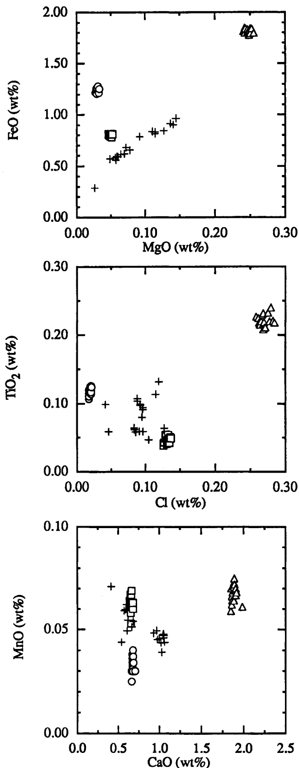
FIGURE 5. Results of replicate analyses performed on three glass inclusions that were used as working standards from one analysis session to another. Plot shows 23 separate analyses of the three working standards (Table 3) collected over a period of eight months by two operators. The circles are data for a glass inclusion from the Esopus Formation at Cherry Valley, New York. The squares are data for a glass inclusion from the Toba Tuff. The triangles are the results for a glass inclusion from Otsuquago Creek bentonite. The plus signs are the results of analyses of different glass inclusions from a single bentonitic tephra from the Devonian Mandata Formation in the Central Appalachian Basin. Note the strong covariation between MgO and FeO and the bimodal distribution of CaO among this population of inclusions. This detail would not be detectable using lower precision electron microprobe techniques.
