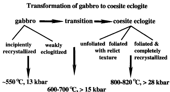
FIGURE 1. Schematic of steps and summarized P-T estimates for transformation of gabbro to coesite eclogite assemblages from Yangkou Beach, eastern China.
