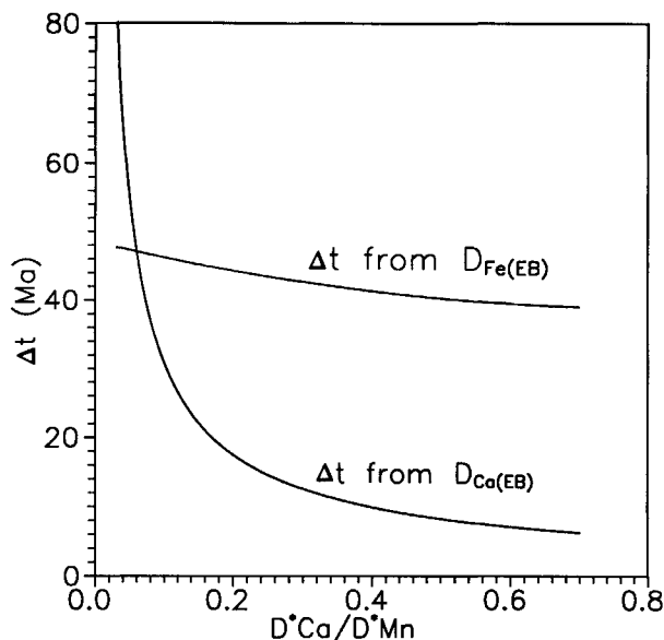
FIGURE 5. Variations of the calculated time scales ( \Delta t ) of biotite-grade metamorphism ( T_{\text{Ch}} = \sim 343^\circ\text{C} ) as functions D_{\text{Fe(EB)}} and D_{\text{Ca(EB)}} , which are derived from assumed values of D_{\text{Ca}}^* . The latter were normalized to D_{\text{Mn}}^* . Convergence of values of \Delta t was obtained at D_{\text{Ca}}^*/D_{\text{Mn}}^* = 0.06 (i.e., D_{\text{Ca}}^* = 9.72 \times 10^{-27} \text{ cm}^2/\text{s} ).
