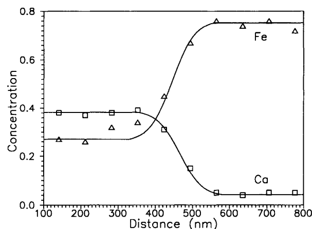
FIGURE 4. Fits of the measured concentration profiles in ATEM of Ca (squares) and Fe (triangles) across the core-overgrowth interface of garnet with Dt = 7.5 \times 10^{-12} \text{ cm}^2 .
