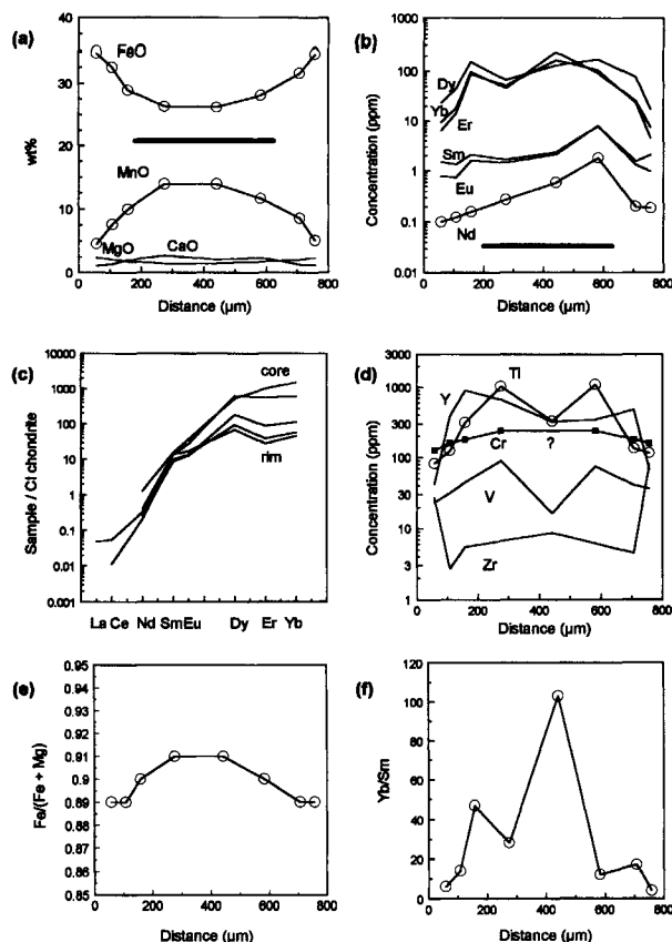
FIGURE 4. Rim-to-rim elemental zonation of a representative GZ garnet (sample 23). Open circles mark positions of SIMS analyses and are the same for each element. Thick lines show inclusion-rich region of crystal. (a) Major element zonation profile determined by EMP at the same positions as the SIMS analyses. (b) REE zonation profile. (c) Chondrite-normalized REE plot of individual SIMS analysis points. (d) Transition element zonation profile. (e) Fe/(Fe + Mg) profile. (f) HREE/LREE profile.
