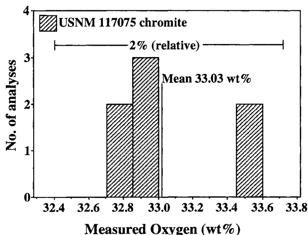
FIGURE 2. Frequency histogram of repetitive O analyses of the USNM 117075 chromite during an analytical session. The chromite has an average O content of 33.03 wt%. The error bar indicates 2% (relative) of the mean.
