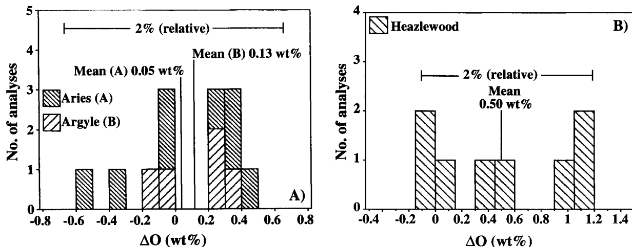
FIGURE 4. (A) Frequency histogram of \Delta O for spinel from the Aries kimberlite and Argyle lamproite. The error bar indicates 2% (relative) of the mean. (B) Frequency histogram of \Delta O
