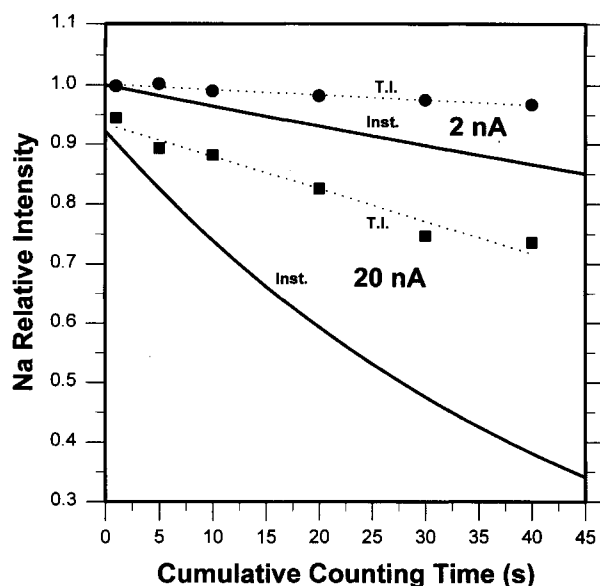
FIGURE 4. Time-integrated (T.I.) vs. instantaneous (Inst.) relative intensities for NaK \alpha X-rays in SM35 glass for 2 nA (circles) and 20 nA (squares) beam conditions.
