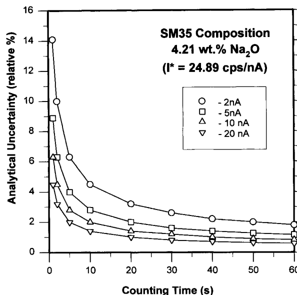
FIGURE 6. Analytical uncertainty [ = 100(N^{1/2}/N ), where N = total counts above mean background] for Na in SM35 glass as a function of counting time. Intensities for calculations are based on the zero-time count rate for \text{NaK}\alpha at 2 nA ( = I^* ), which was derived by exponential fit to the raw data in Figure 1a.
