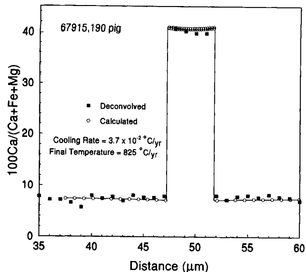
FIGURE 9. Measured (deconvolved) and calculated profiles in a traverse across pigeonite host and augite lamella from sodic ferrogabbro 67915,190. Value of \epsilon is 0.55.
