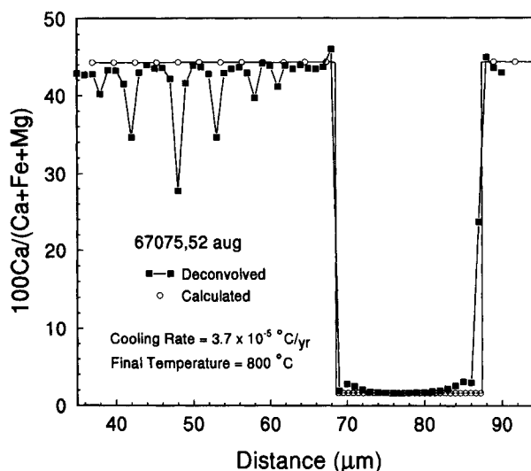
FIGURE 5. Measured (deconvolved) and calculated profiles in a traverse across a pigeonite lamella and augite host in anorthosite 67075,52. Deconvolution factor \epsilon = 0.55 . Second-generation lamellae were ignored in the modeling.
