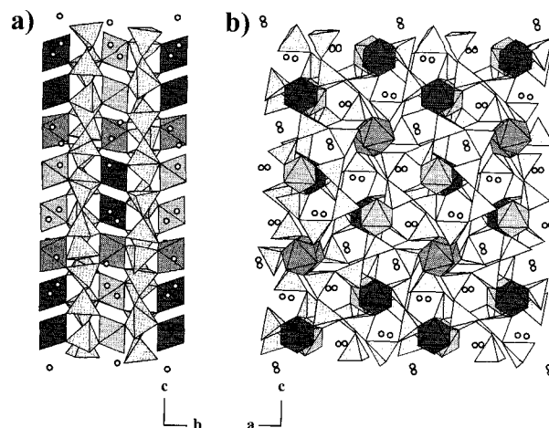
FIGURE 2. Polyhedral representations of the structure of \text{Na}_6\text{Si}_3[\text{Si}_9\text{O}_{27}] viewed along [100] (a) and [010] (b). Shading of octahedra is light for \text{Si}_2\text{O}_6 , moderate for \text{Si}_3\text{O}_6 , and heavy for \text{Si}_4\text{O}_6 . Open circles are Na positions. Note that the layers of collapsed nine-membered rings of \text{SiO}_4 tetrahedra are in ABA... packing along [010]. Also, octahedra, interspersed with unoccupied trigonal prisms, form columns along [010], with alternating \text{Si}_2\text{O}_6 and \text{Si}_3\text{O}_6 in one column and \text{Si}_4\text{O}_6 alone in another.
