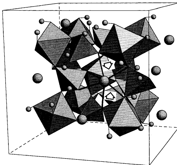
FIGURE 4. Portion of the katoite unit cell, illustrating the framework of corner-sharing tetrahedra and octahedra and the orientation of the O-H vectors. The large solid sphere in the center of the drawing represents Ca, which is coordinated to eight O atoms located at the corners of a distorted cube (dodecahedron). The four short Ca-O bonds are opposite the two edges shared between the dodecahedron and tetrahedron. For clarity, only two of the four long bonds are shown. The O4 atom is displaced in the direction of Ca (arrows), as octahedra and tetrahedra undergo rigid-body rotations at high pressure.
