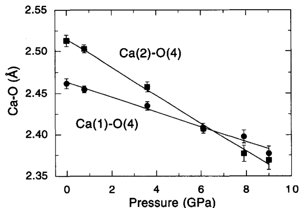
FIGURE 5. Variation of two unique Ca-O distances in the dodecahedron as a function of pressure.
