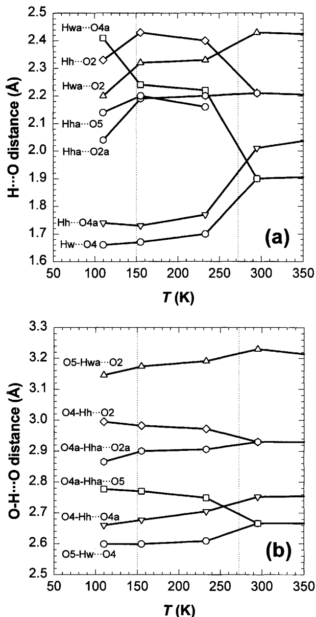
FIGURE 5. Plot of hydrogen-bond distances in lawsonite (values from Table 1) vs. temperature. (a) H...O distances. (b) O-H...O straight distances.
