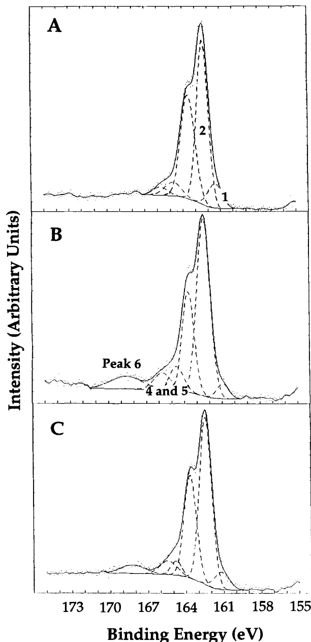
FIGURE 5. XPS S 2p spectra (eight scans). Fitted peaks are numbered in A and B. Bottom solid line is background, top solid line is sum of background and fitted peaks. (A) Fresh surface, (B) 1 d in air, (C) 5 d in air.
