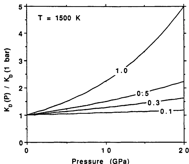
FIGURE 5. Equilibrium constant, K_D , for Fe-Mg distribution in a ferromagnesian silicate varies as a function of pressure for different volumes of disordering ( \Delta V_{\text{dis}} in cubic centimeters per mole), as marked on each curve. Curves were calculated for a temperature of 1500 K. At lower temperatures the effect of pressure on K_D is somewhat larger for a given \Delta V_{\text{dis}} (see Eq. 10).
