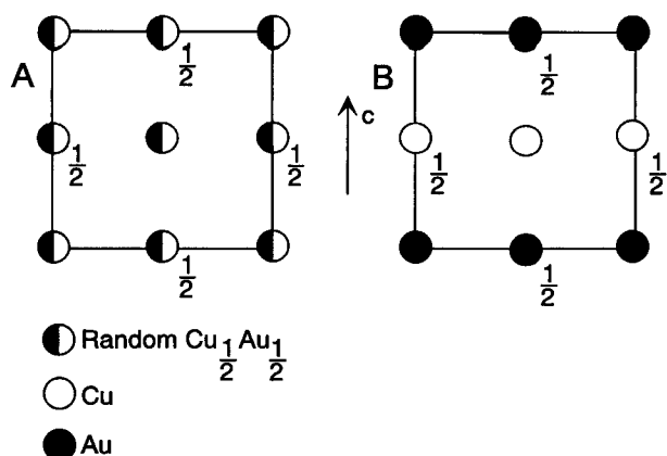
FIGURE 2. The structure of \text{CuAu} : (A) disordered form, space group Fm\bar{3}m ; (B) ordered form, space group Pm\bar{3}m . The fully ordered form is approximately 0.8% denser than the fully disordered form.
