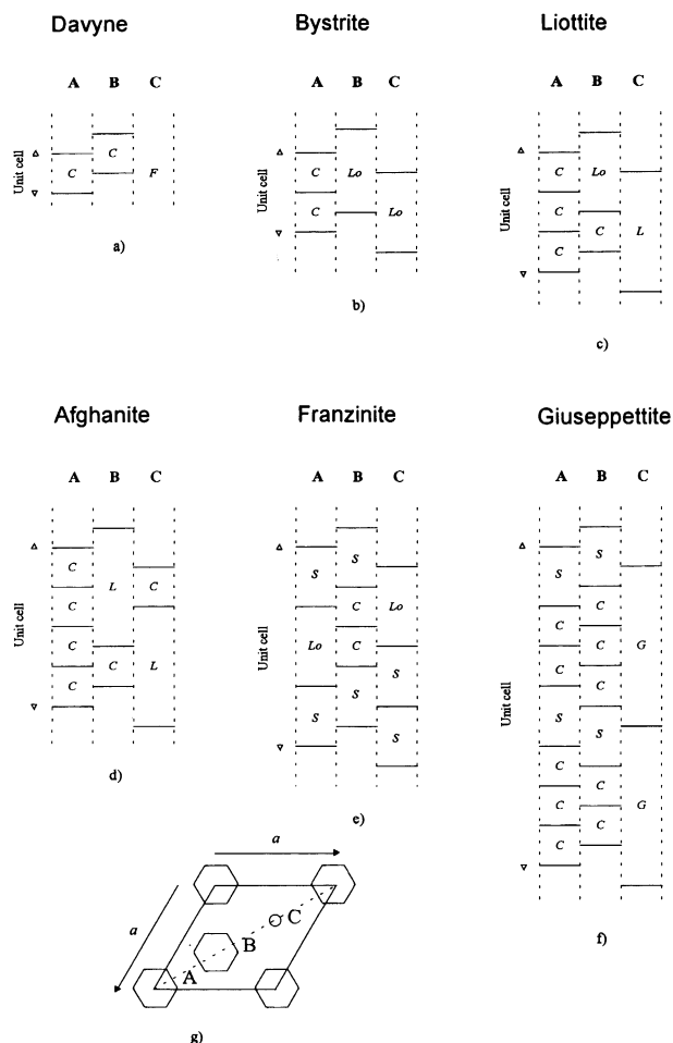
FIGURE 8. Schematic representation of the frameworks of cancrinite-like minerals: (a) davynite-type, (b) bystrite, (c) liottite, (d) afghanite, (e) franzinite, (f) giuseppettite. Solid lines represent six-membered rings of Si,Al tetrahedra. The dotted lines identify the various structural units generated by the different stacking sequences. F = free channel, Lo = losod cage, C = cancrinite cage, L = liottite cage, S = sodalite cage, G = giuseppettite cage. (g) Schematic [001] drawing of the framework of an AB-type structure. It is possible to observe the three different positions (A = 0, 0, z; B = \frac{2}{3} , \frac{1}{3} , z; C = \frac{1}{3} , \frac{2}{3} , z) occupied by the centers of the six-membered rings of Si,Al tetrahedra stacked along c.
