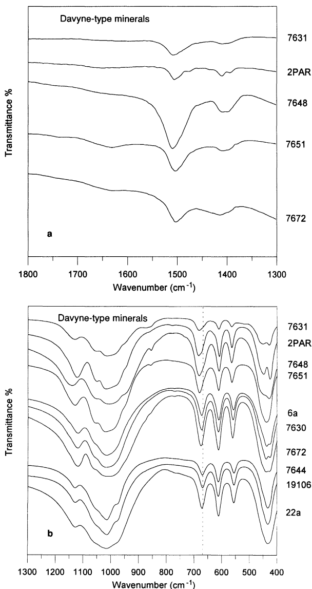
FIGURE 1. IR spectra of davyne-type minerals. (a) Range 1800–1300 \text{cm}^{-1} . The two distinct groups of bands in the 1500–1400 \text{cm}^{-1} zone are possibly due to \text{CO}_3 groups. Samples without bands in this range are not reported for clarity. (b) Range 1300–400 \text{cm}^{-1} . The samples are arranged, from bottom to top, with increasing frequency of the first band of the triplet located at 700–550 \text{cm}^{-1} .
