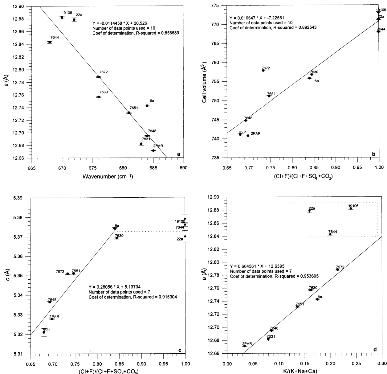
FIGURE 5. (a) Correlation between the a cell dimension and the first band of the triplet located in the range 700–550 cm -1 of the davyne-type spectra. (b) Cell volume vs. Cl content of davyne-type minerals. (c) Relationship between the c parameter and the Cl content of davyne-type minerals. The expansion limit is reached at about 0.85. Further increases in Cl content do not seem to expand the c cell parameter. The quadridavnye samples
