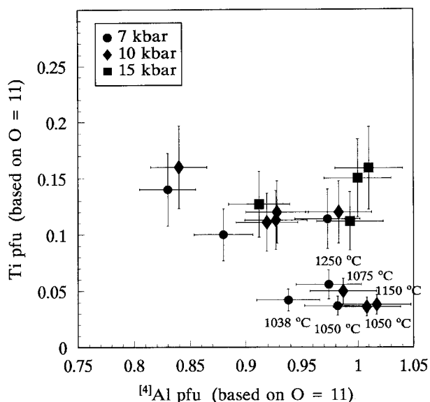
FIGURE 3. Ti pfu vs. 4 Al pfu, suggesting that the Ti-Tschermak's substitutional mechanism ( \text{Ti}^{4+}\text{Al}_2\text{Mg}_{-1}\text{Si}_{-2} ) does not occur in the phlogopite from these experiments. Data points not labeled with a temperature are for experiments performed at T \geq 1250 °C.
