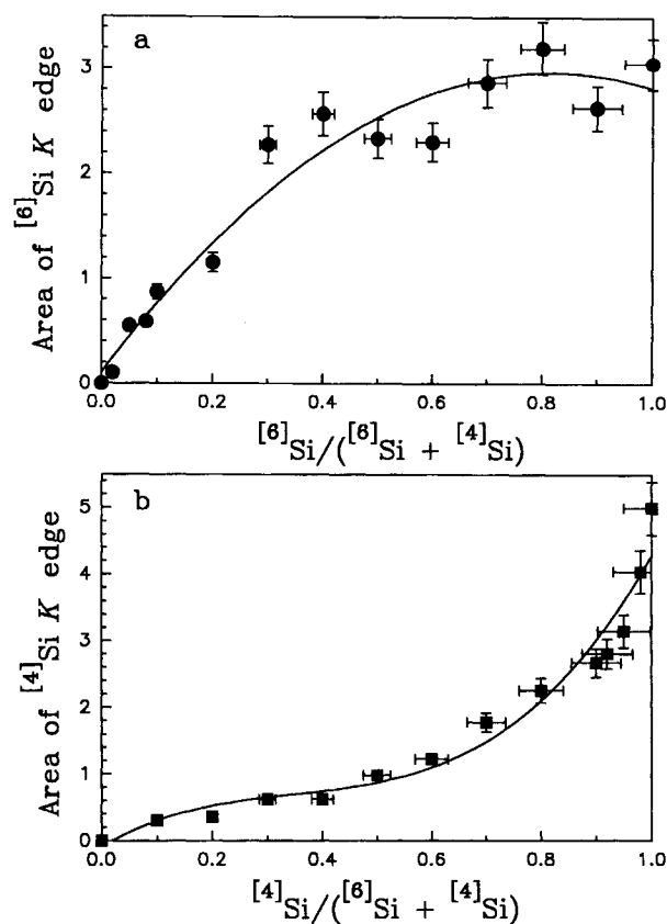
FIGURE 3. The integrated areas (or relative intensities) of [ 6 Si] (dots) (a) and [ 4 Si] (squares) (b) edge peaks correlated with atomic proportion of species in model composite materials. Error in composition was estimated to be about 5%, and the errors for the integrated areas were estimated to be about 8%. The solid lines were fitted by least-squares regression.
