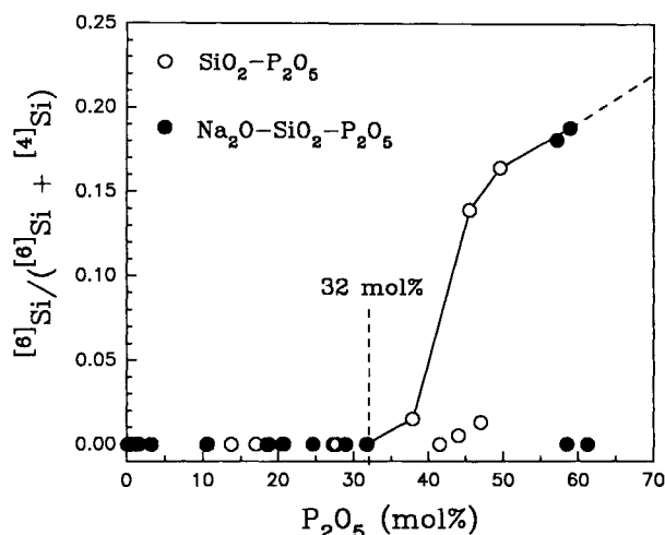
FIGURE 7. Atomic proportion of ^{46}\text{Si} as a function of \text{P}_2\text{O}_5 content in \text{SiO}_2\text{-P}_2\text{O}_5 (open circles) and \text{Na}_2\text{O-SiO}_2\text{-P}_2\text{O}_5 (solid circles) glasses. The threshold value of \text{P}_2\text{O}_5 for stabilizing ^{46}\text{Si} in these glasses appears to be about 32 mol%. Data for \text{P}_2\text{O}_5 contents of less than 30 mol% are from Li et al. (1995a).
