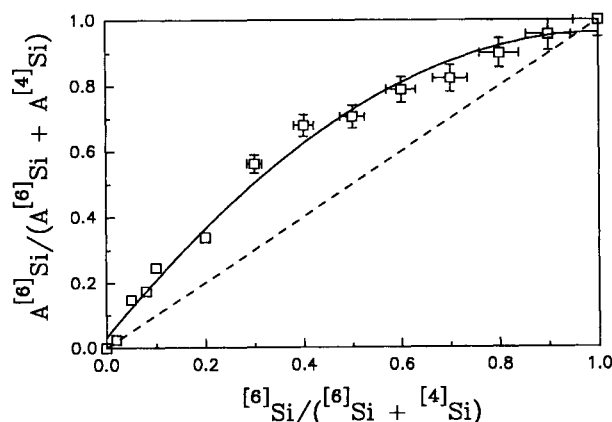
FIGURE 4. Correlation of peak area ratio for ^{16}\text{Si} and ^{14}\text{Si} with atomic proportion of species in model composite materials. Error in the area ratio was estimated to be about 5%. The solid line was fitted with experimental data (open squares) by least-squares regression, and the dashed line represents the ideal proportional correlation. An empirical equation was derived for the model materials and may be used for the quantification of ^{16}\text{Si} and ^{14}\text{Si} in glasses and other materials of unknown structure.
