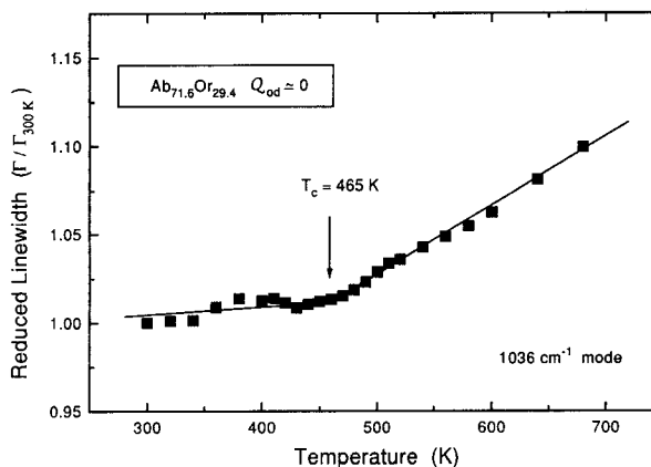
FIGURE 13. The change in the temperature dependence of the reduced line width of the 1036 \text{cm}^{-1} mode in \text{Ab}_{71.6}\text{Or}_{29.4} ( Q_{\text{od}} = 0 ) at 465 K corresponds to the structural phase transition C2/m-C\bar{1} .
