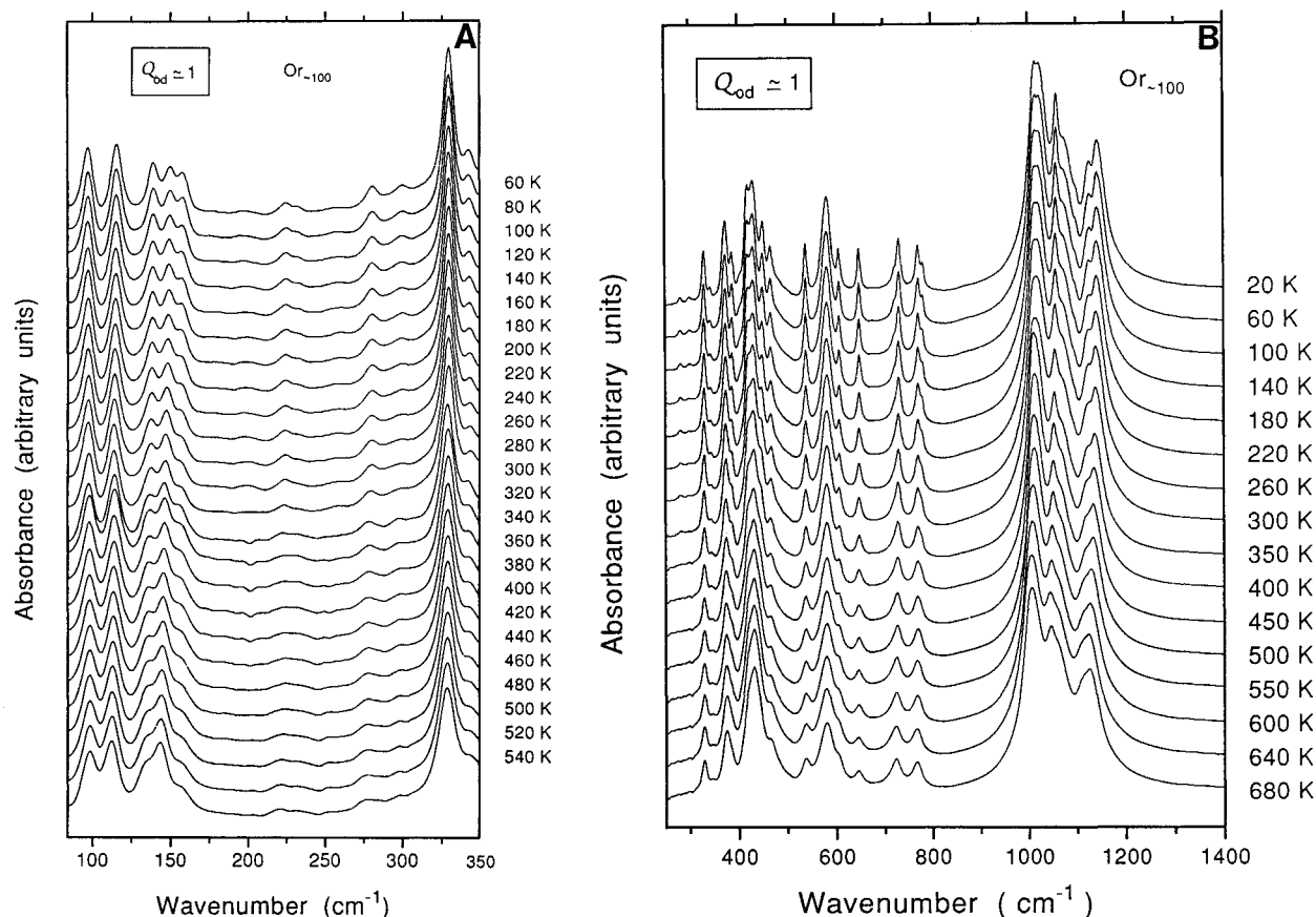
FIGURE 4. Temperature evolution of infrared absorption spectra of microcline ( \text{Or}_{100} , Q_{\text{od}} \approx 1 ). Low- and high-temperature spectra in the spectral range 80–350 \text{cm}^{-1} (A) and 250–1400 \text{cm}^{-1} (B).
