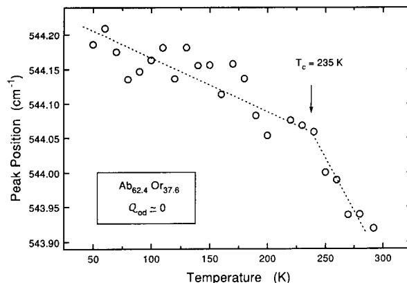
FIGURE 12. Thermal frequency shift of the 544 \text{cm}^{-1} phonon with a structural phase transition C2/m-C\bar{1} at T_c = 235 K ( \text{Ab}_{62.4}\text{Or}_{37.6} , Q_{\text{od}} = 0 ).
