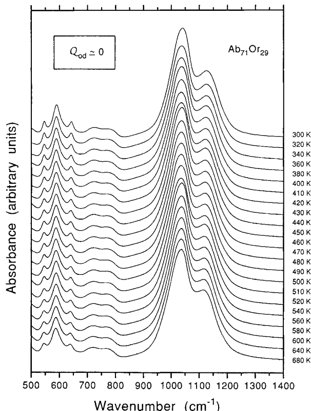
FIGURE 7. Phonon spectra of \text{Ab}_{71}\text{Or}_{29} ( Q_{\text{od}} \approx 0 ) at high temperatures (490–1400 \text{cm}^{-1} ).
