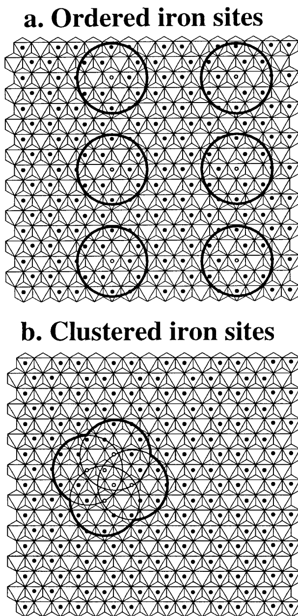
FIGURE 8. Schematic two-dimensional representations of an ideal dioctahedral sheet. Solid dots show Al sites, open dots show Fe sites. (a) Fe sites are regularly ordered in a sheet with an average Al:Fe ratio of 27:1. The bold circles represent wipeout circles with a radius of 6 Å. In this example, 56% of the Al sites are outside the circle. (b) Fe sites clustered in the sheet also have an average Al:Fe ratio of 27:1. In this scenario, 82% of the Al sites are outside the circle. The model discussed in the text is different in that it offers a three-dimensional consideration of dioctahedral sites.
