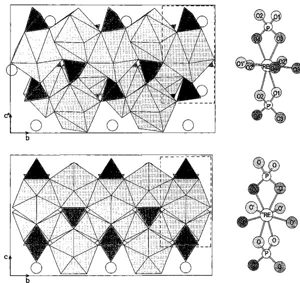
Fig. 2. Atomic arrangements of monazite ( top ) and xenotime ( bottom ). Polyhedral projections down [100] illustrate the similarity between the two atomic arrangements. Ball and stick chains and atomic nomenclature for each structure are depicted to right; ball and stick depictions are rotated about c* for clarity of viewing. Dashed line outlines polyhedron-tetrahedron chain illustrated on right. Open circles represent RE atoms.
