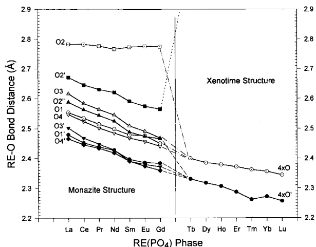
Fig. 4. Selected RE-O bond distances in synthetic RE(PO 4 ) phases.
