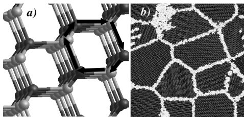
Figure 1. a) Definition of a ring. The shortest closed path (marked by black arrows) includes 3 Si-C pairs and constitutes a 3-fold ring. In a zinc-blende structure, each atom participates in 12 unique 3-fold rings. b) Crystalline atoms (grey) and grain boundaries (white) in MD sample 10.5nm sintered in 7GPa based on the ring analysis criterion.
