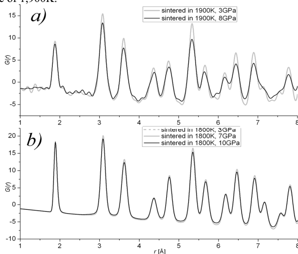
Figure 2. Reduced PDF, G(r) , of SiC ceramics: experimental (a) and from MD simulation (b). In both plots the grey line corresponds to lower sintering pressures as compared to the data marked with a black line. 3 GPa and 7 GPa lines in (b) are very similar and cannot be distinguished.
