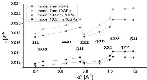
Figure 3. Williamson-Hall plot for data calculated from MD models.
