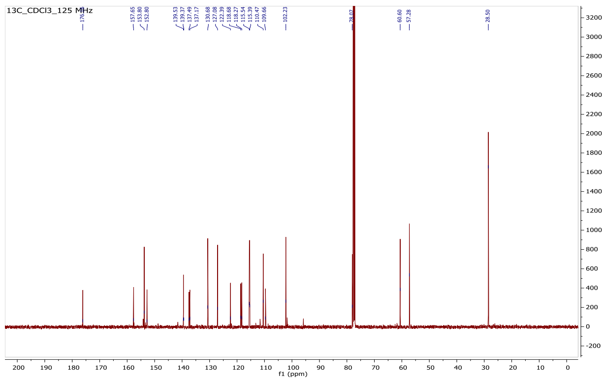
Figure S2 ^{13}\text{C} NMR spectrum of (1) observed at 125 MHz for \text{CDCl}_3 solvent at 25^\circ\text{C} .
