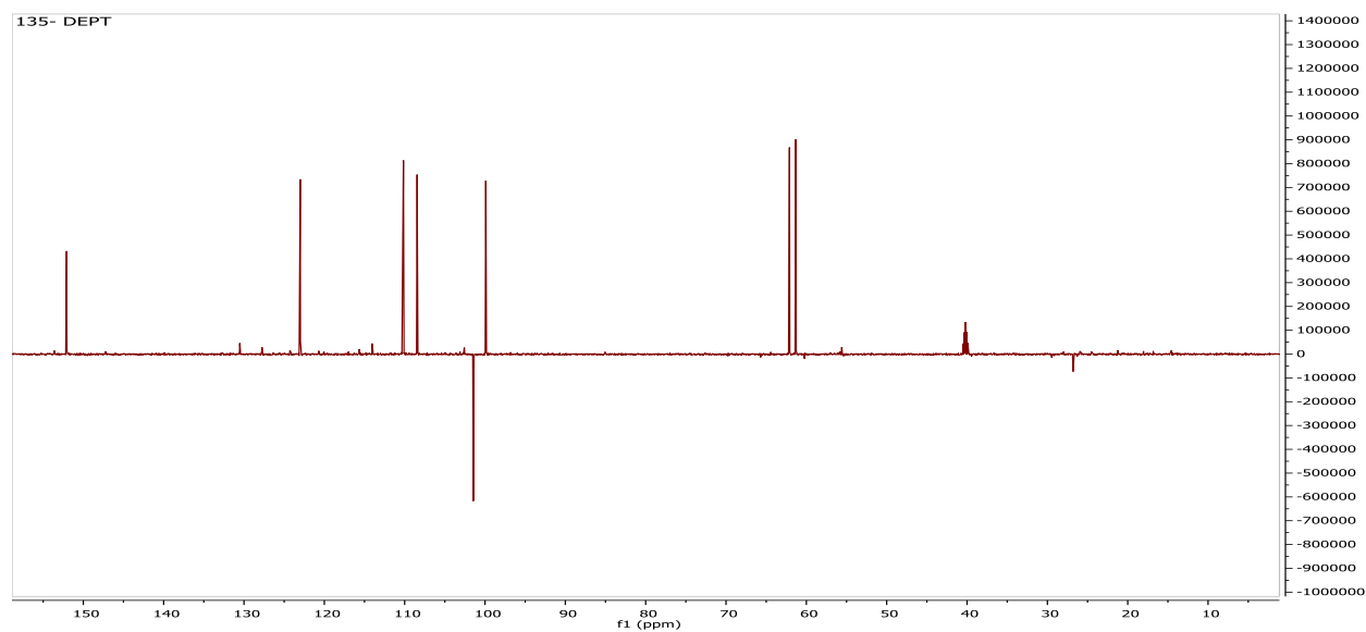
Figure S23 ^{135}\text{DEPT} (4) observed at 125 MHz for \text{CDCl}_3 solvent at 25^\circ\text{C} .
