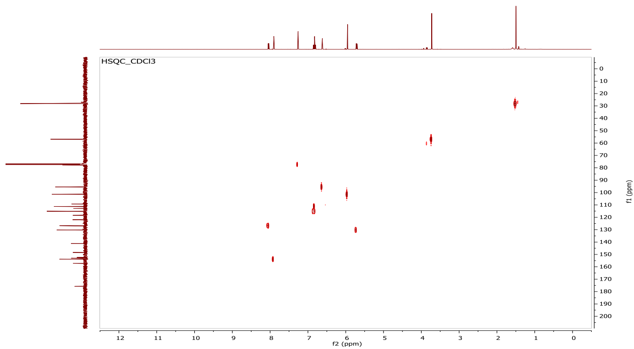
Figure S10 COSY (2) observed at 500 MHz for \text{CDCl}_3 solvent at 25^\circ\text{C} .
