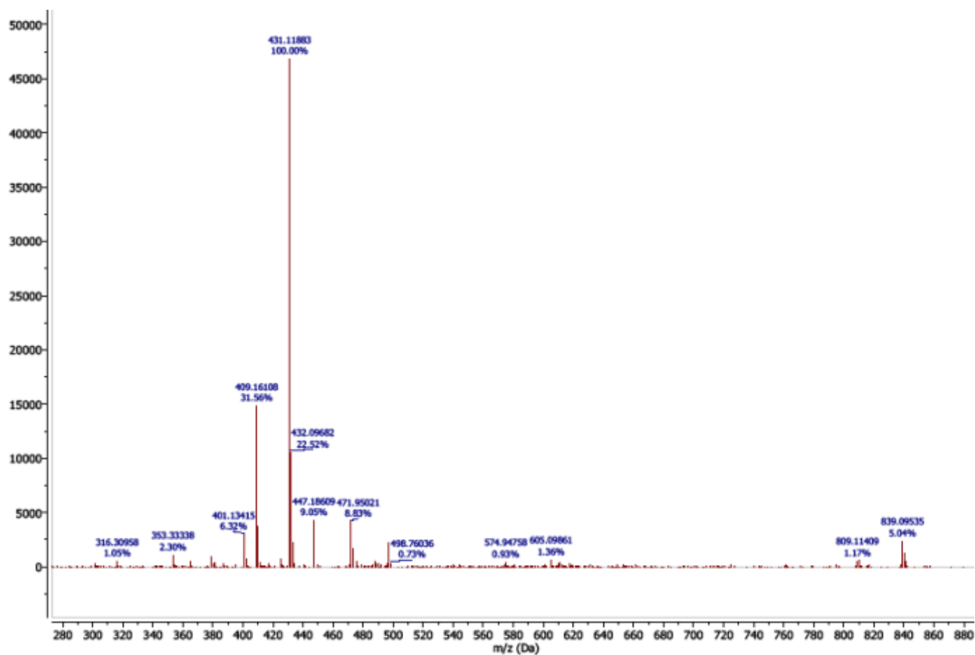
Figure S19 The ESI-MS Spectrum of (3)
