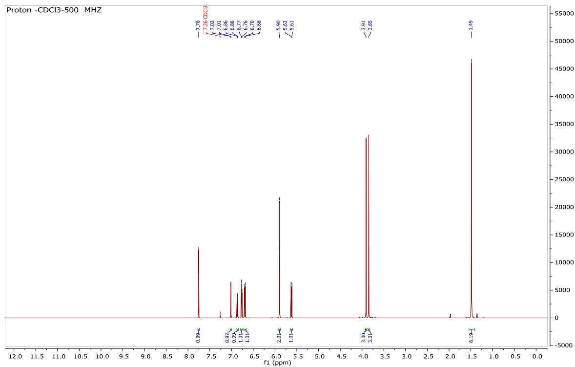
Figure S14 1 H NMR spectrum of (3) observed at 500 MHz for CDCl 3 solvent at 25 0 C.
