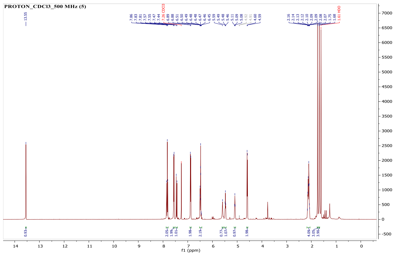
Figure S28 1 H NMR spectrum of (5) observed at 500 MHz for CDCl 3 solvent at 25 0 C.
