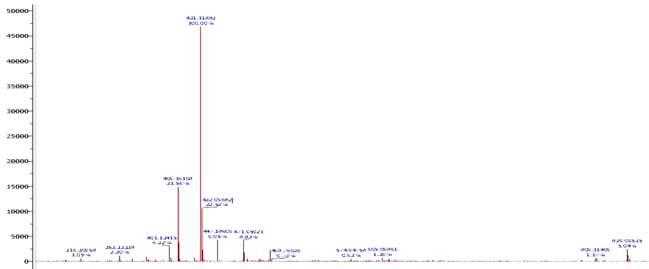
Figure S5 HMBC spectrum of (1) observed at 500 MHz and 125 MHz for CDCl 3 solvent at 25 o C
