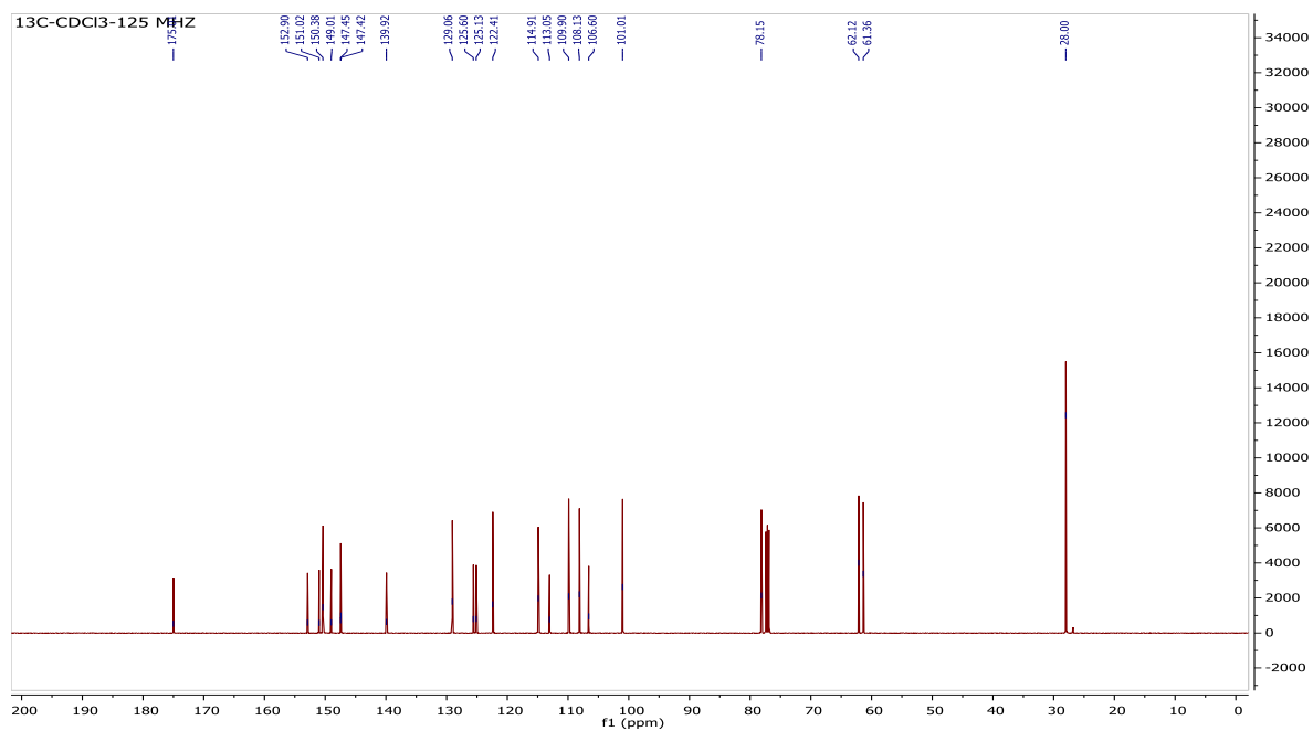
Figure S15 ^{13}\text{C} NMR spectrum of (3) observed at 125 MHz, \text{CDCl}_3 solvent at 250C.
