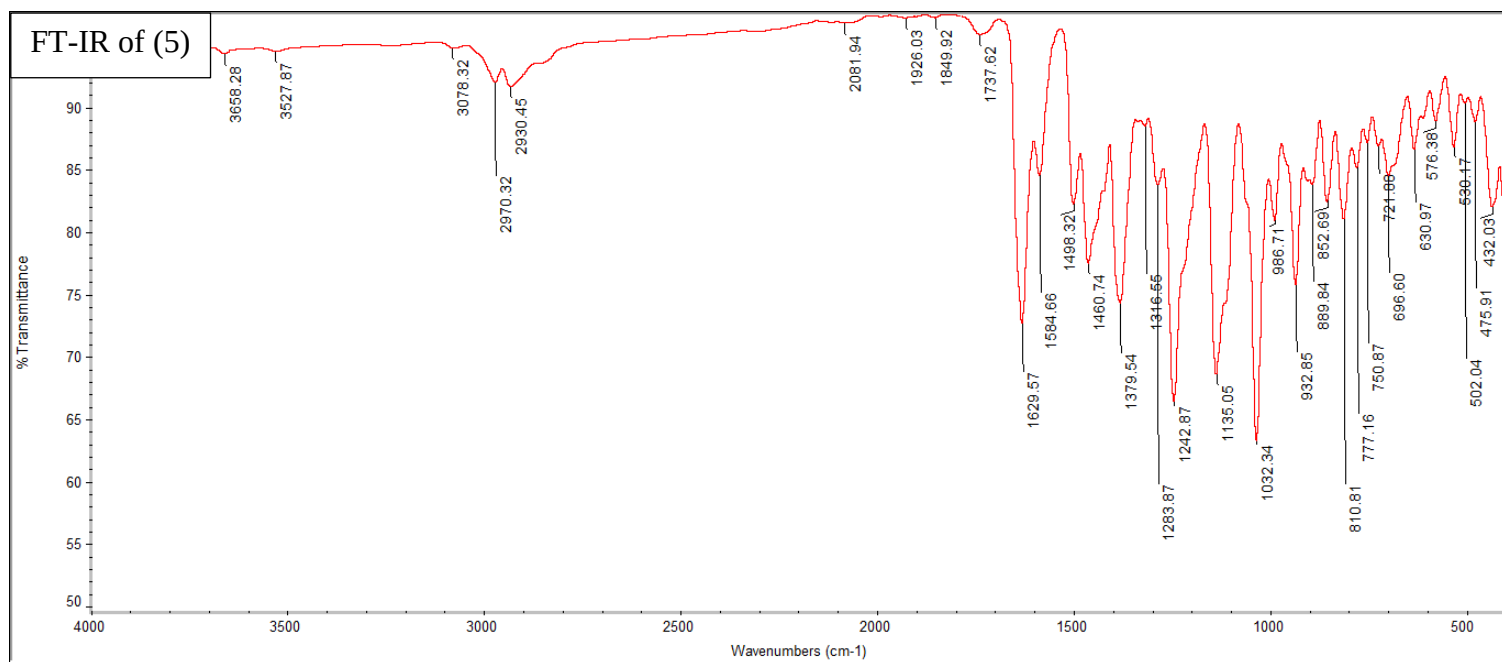
Figure S35 FT-IR spectra of compound of (5)
