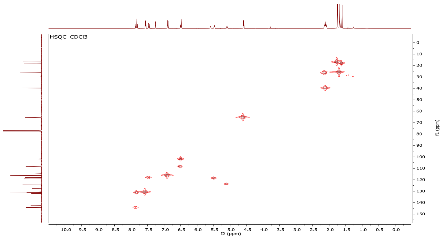
Figure S32 HSQC spectrum of (5) observed at 500 MHz and 125MHz for \text{CDCl}_3 solvent at 25^\circ\text{C} .
