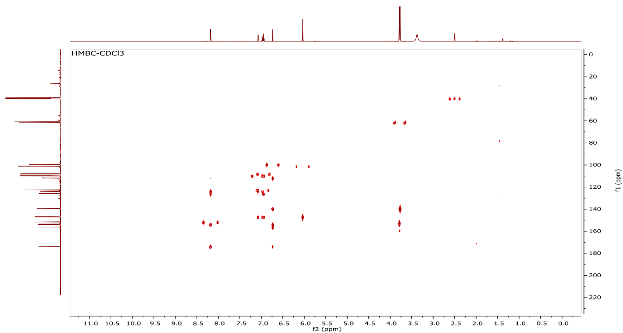
Figure S26 HMBC spectrum of (4) observed at 500 MHz and 125MHz for CDCl 3 solvent
