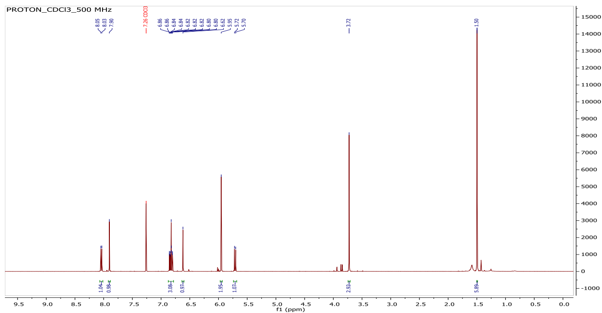
Figure S8 1 H NMR spectrum of (2) observed at 500 MHz for CDCl 3 solvent at 25 0 C.
