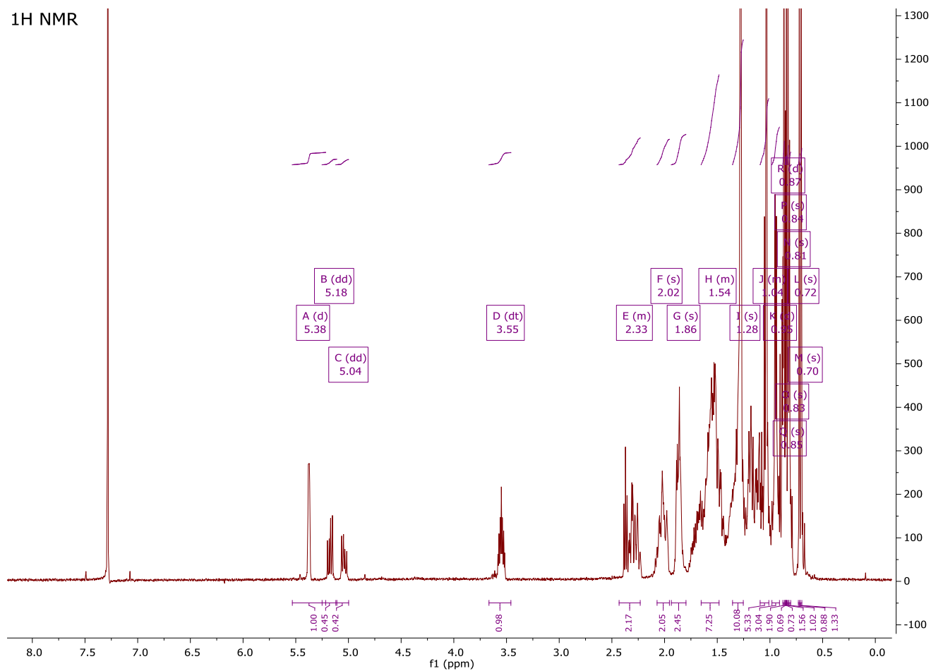
Figure S36 1 H NMR spectrum of (6) observed at 500 MHz for CDCl 3 solvent at 25 0 C.
