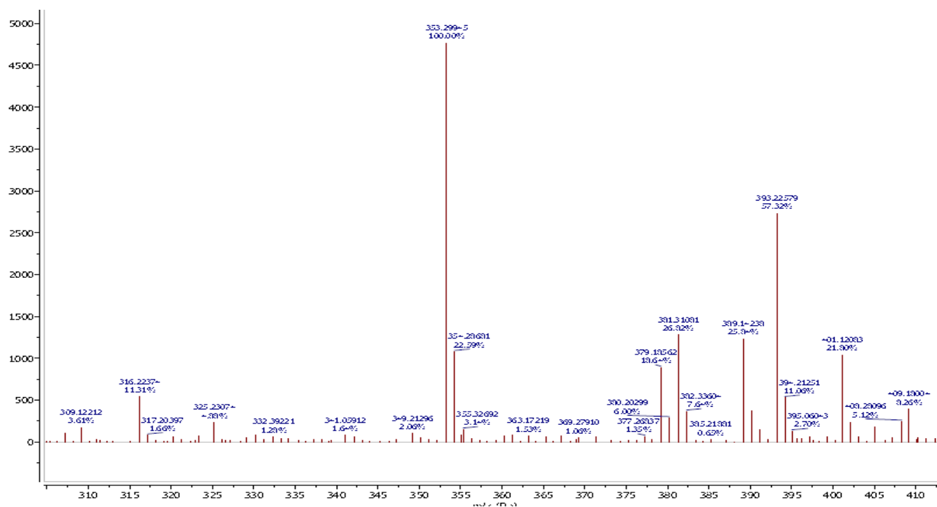
Figure S34 The ESI-MS Spectrum of (5)
