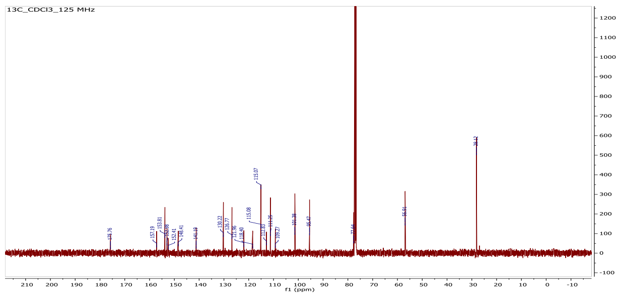
Figure S9 13 C NMR spectrum (2) observed at 125 MHz for CDCl 3 solvent at 25 0 C
