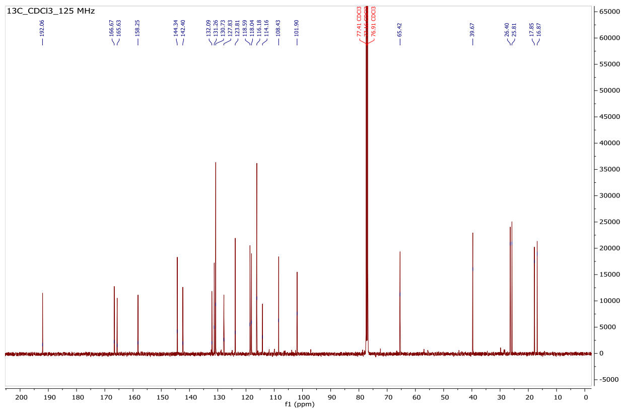
Figure S29 13 C NMR spectrum of (5) observed at 125 MHz for CDCl 3 solvent at 25 0 C .
