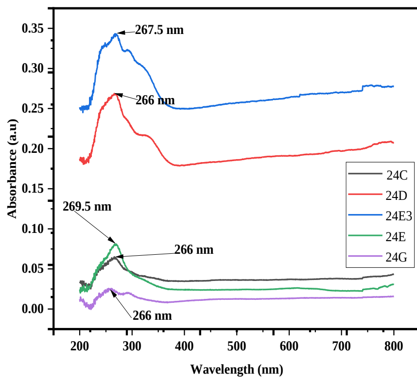
Figure S38 UV spectra of compound of (1-5)
