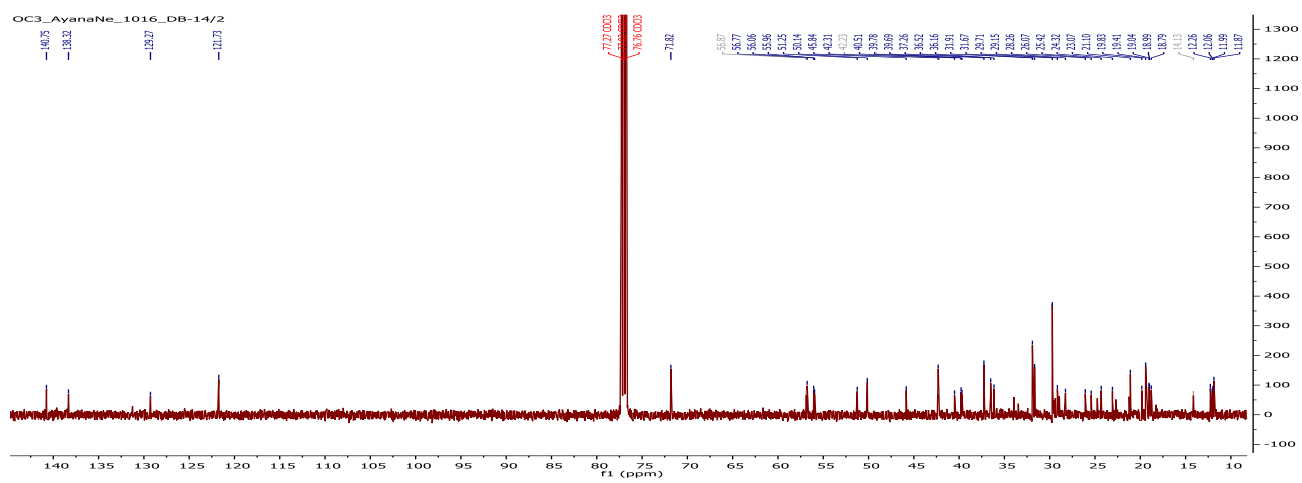
Figure S37 13 C NMR spectrum of (6) observed at 125 MHz for CDCl 3 solvent at 25 0 C.
