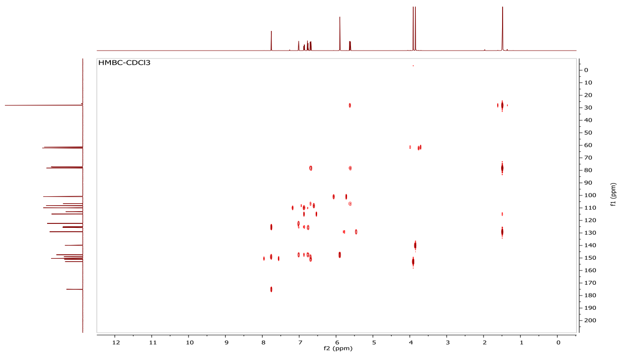
Figure S18 HMBC spectrum of (3) observed at 500 MHz and 125 MHz for \text{CDCl}_3 solvent at 25^\circ\text{C} .
