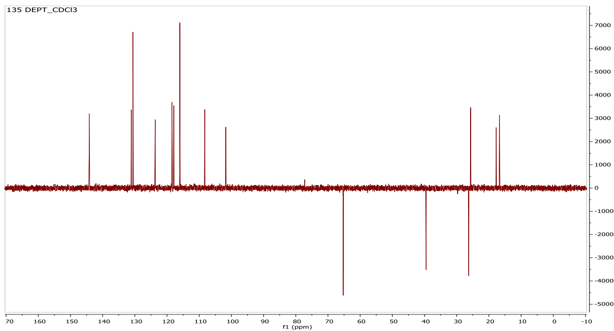
Figure S31 135 DEPT (5) observed at 125 MHz for \text{CDCl}_3 solvent at 25^\circ\text{C} .
