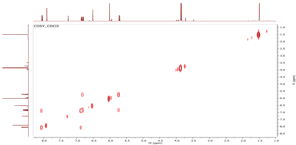
Figure S2 ^{13}\text{C} NMR spectrum of (1) observed at 125 MHz for \text{CDCl}_3 solvent at 25^\circ\text{C} .
