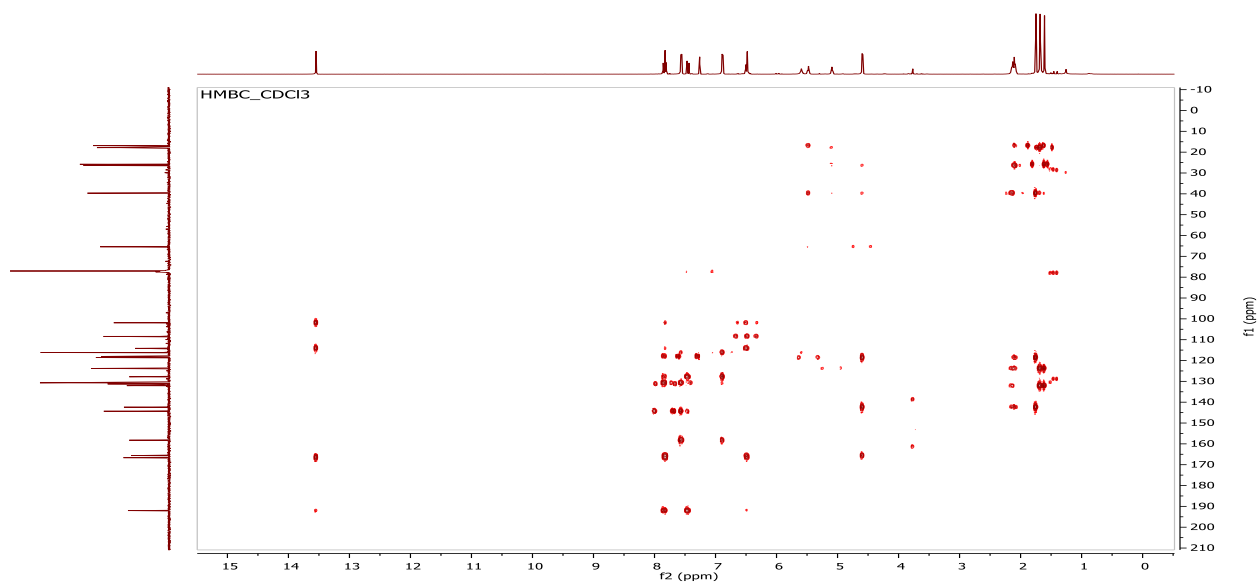
Figure S33 HMBC spectrum of (5) observed at 500 MHz and 125 MHz for \text{CDCl}_3 solvent
