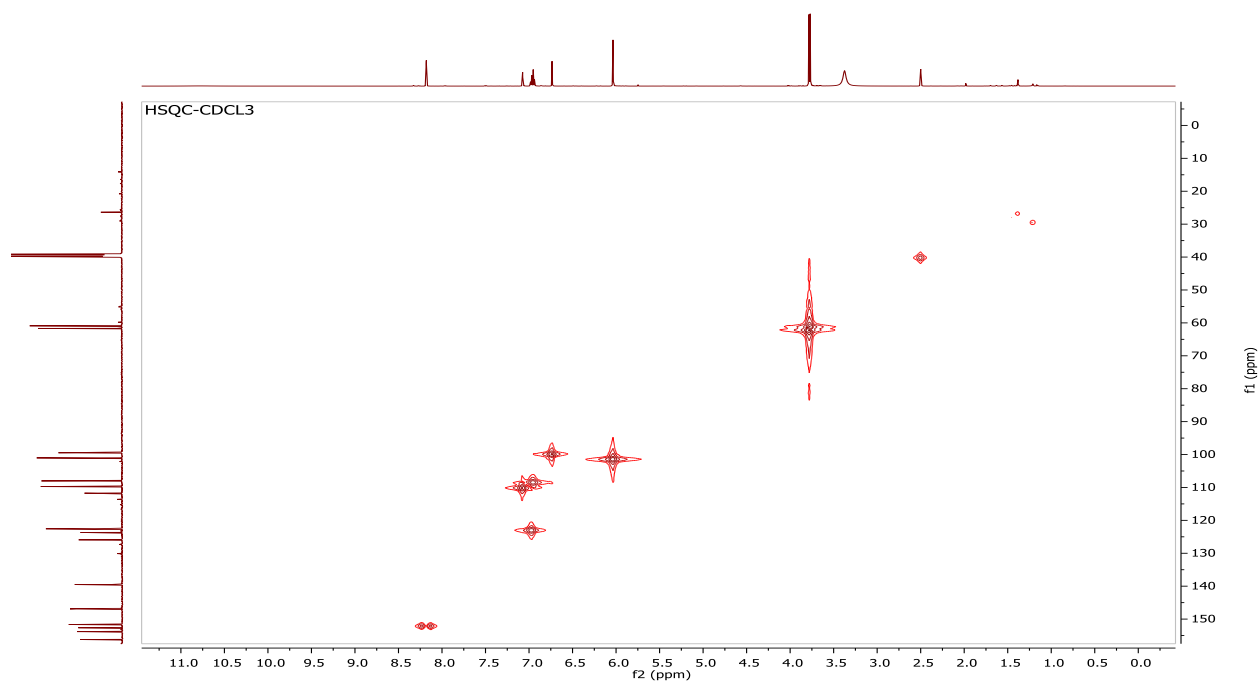
Figure S24 COSY spectrum of (4) observed at 500 MHz for CDCl 3 solvent at 25 0 C.
