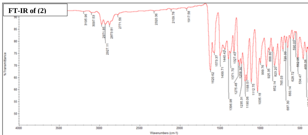
Figure S13 FT-IR spectra of compound (2)
