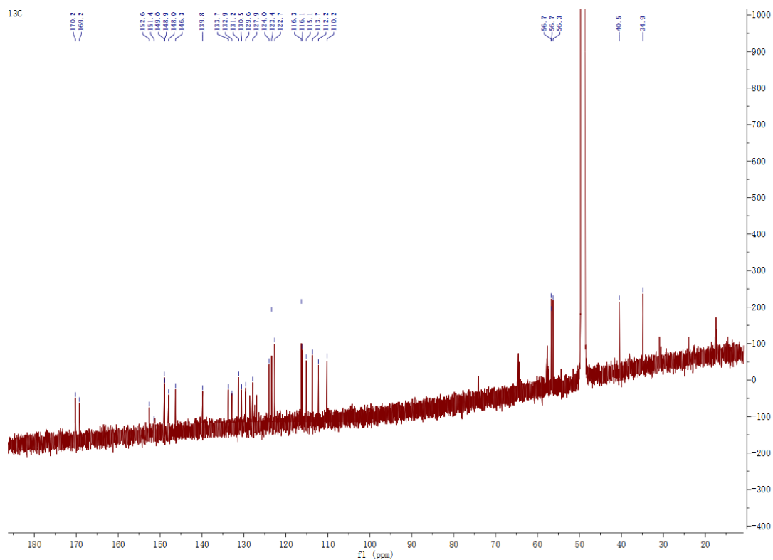
Fig. S5. 13 C NMR (150 MHz) spectrum of oleraisoindole B in methanol- d 4
