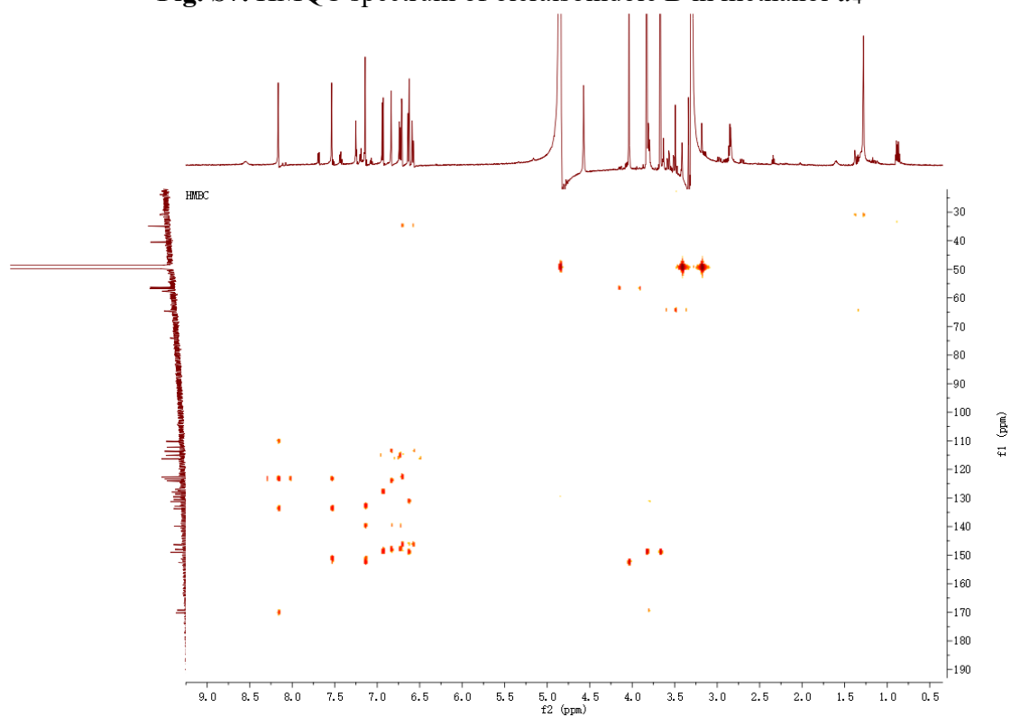
Fig. S7. HMQC spectrum of oleraisoindole B in methanol- d_4
