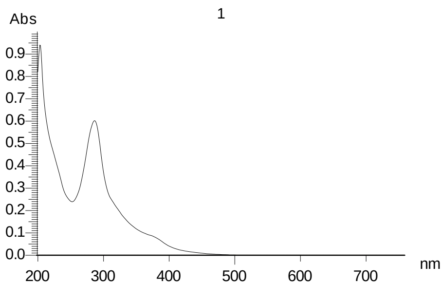
Fig. S2. UV spectrum of oleraisoindole B in methanol- d_4
