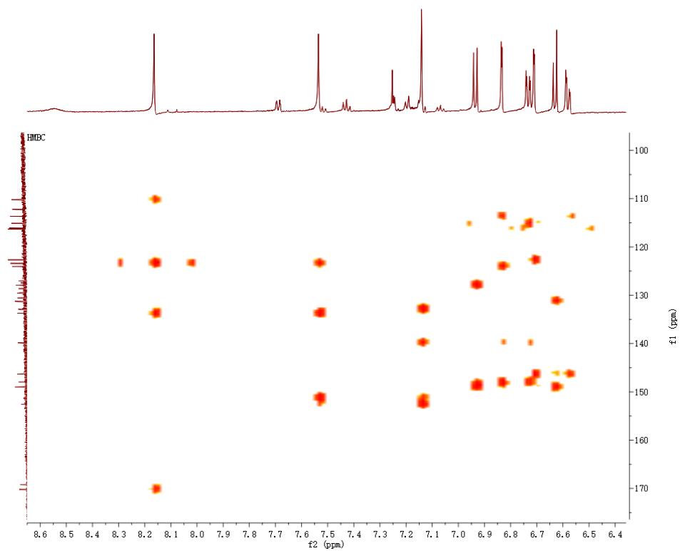
Fig. S8. HMBC spectra of oleraisoindole B in methanol- d_4
