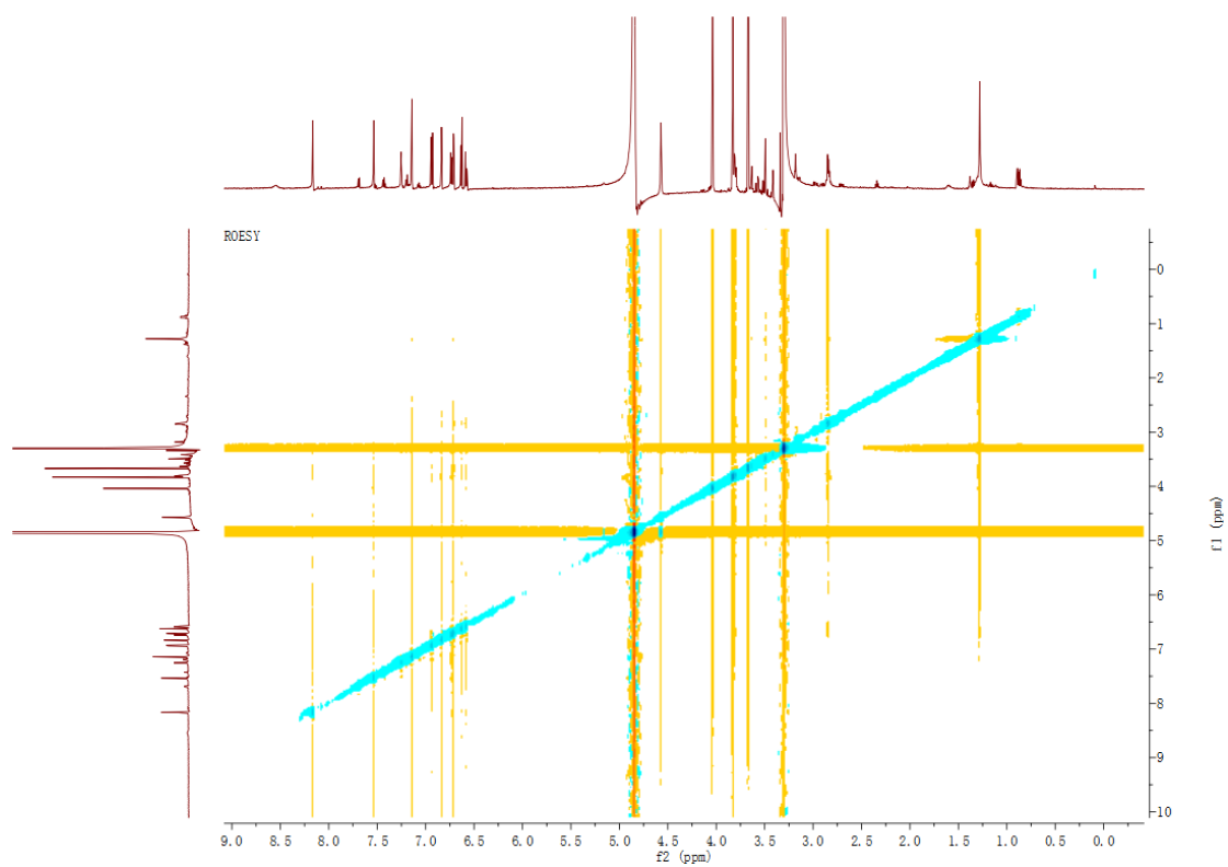
Fig. S10. ROESY spectrum of oleraisoindole B in methanol- d_4
