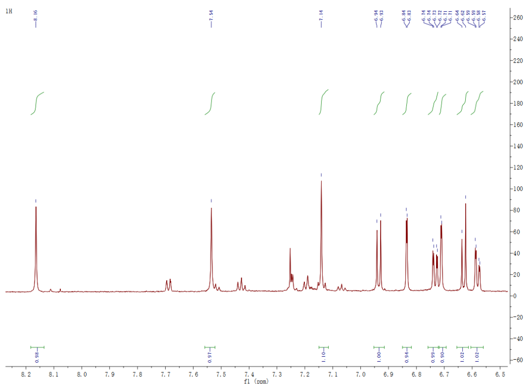
Fig. S4. 1 H NMR (600 MHz) spectra of oleraisoindole B in methanol- d 4
