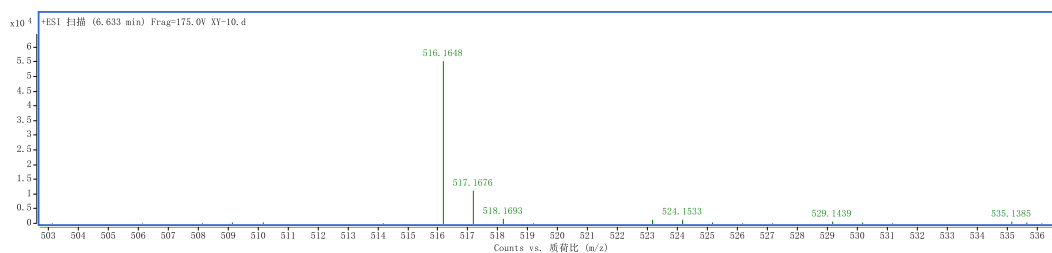
Fig. S1. UHPLC-ESI-Q-TOF/MS of oleraisoindole B in methanol- d_4
