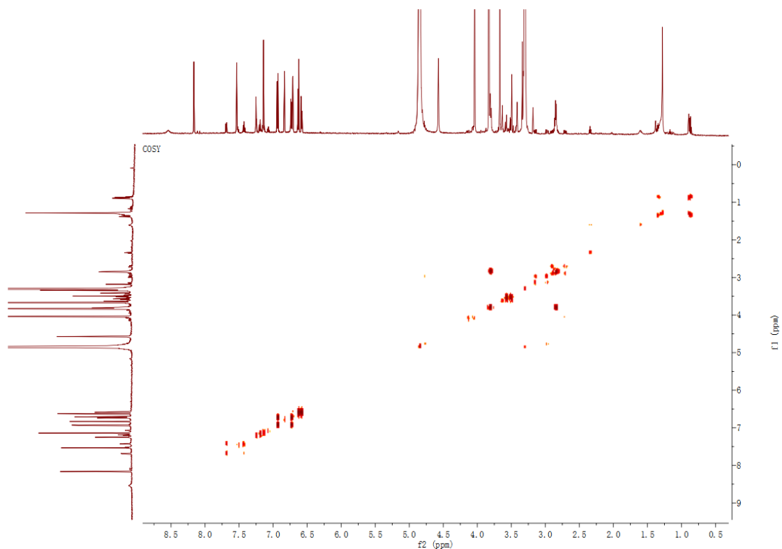
Fig. S9. ^1\text{H} - ^1\text{H} COSY spectrum of oleraisoindole B in methanol- d_4
