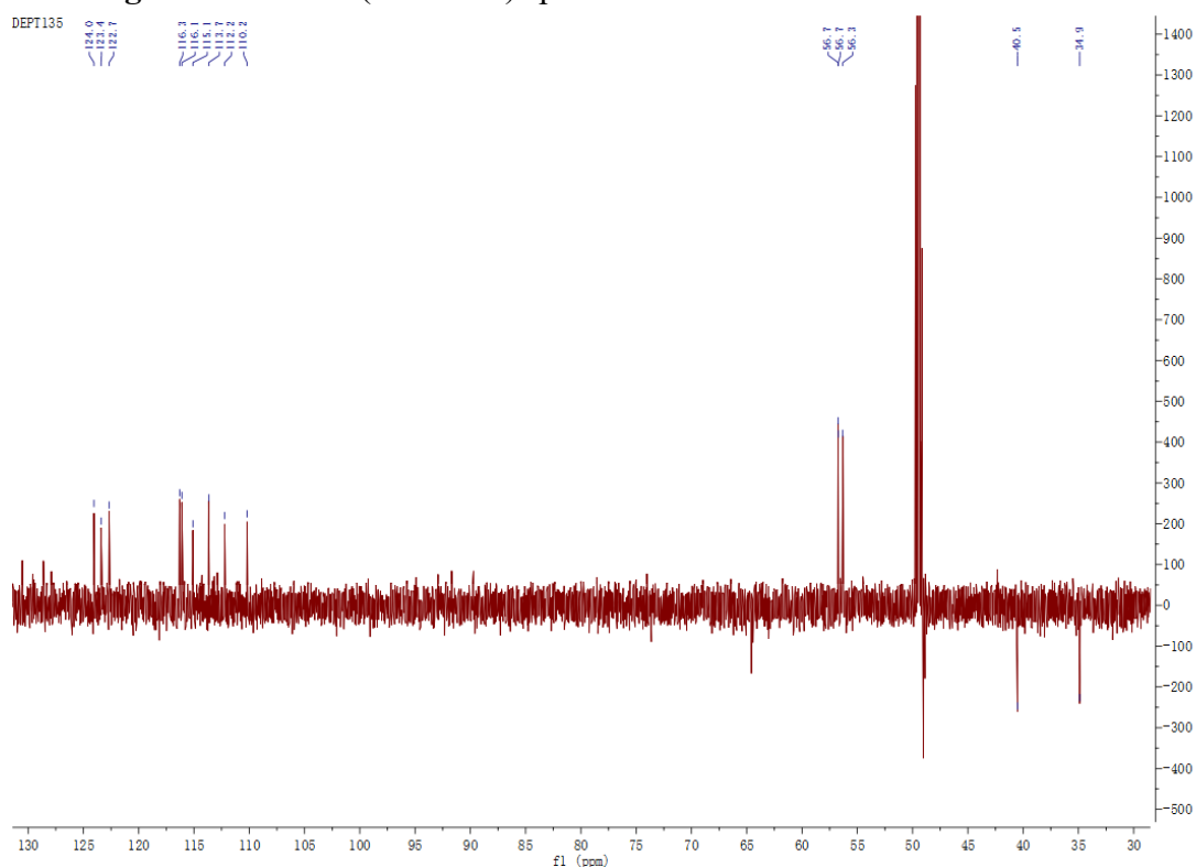
Fig. S6. DEPT spectrum of oleraisoindole B in methanol- d 4
